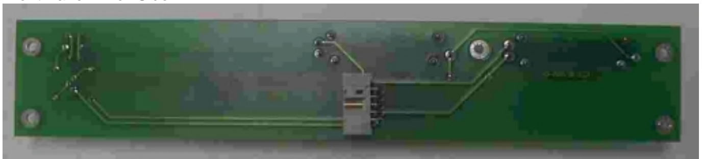
Front Panel – Foil Side
