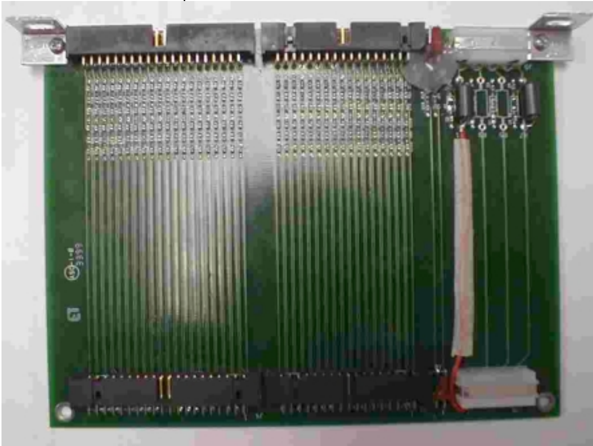
Drive Filter Board – Component Side
