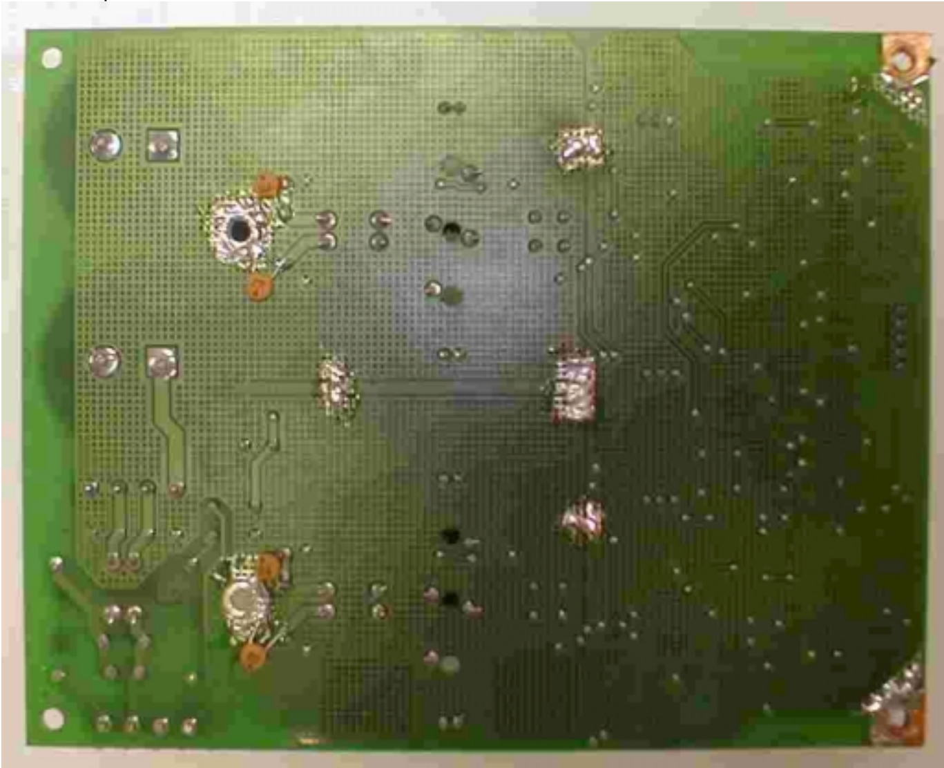
Power Amp – Foil Side
