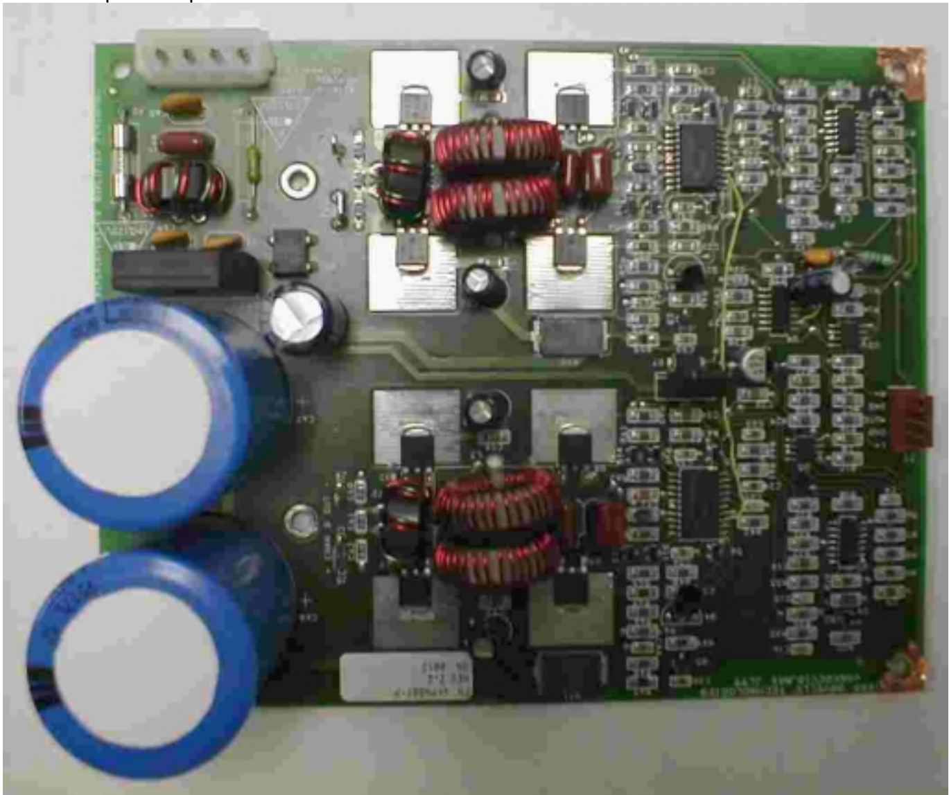
Power Amp – Component Side
