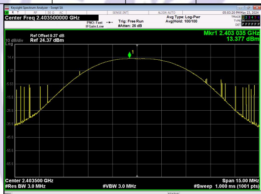
Peak Output Power FSK_Channel 00
