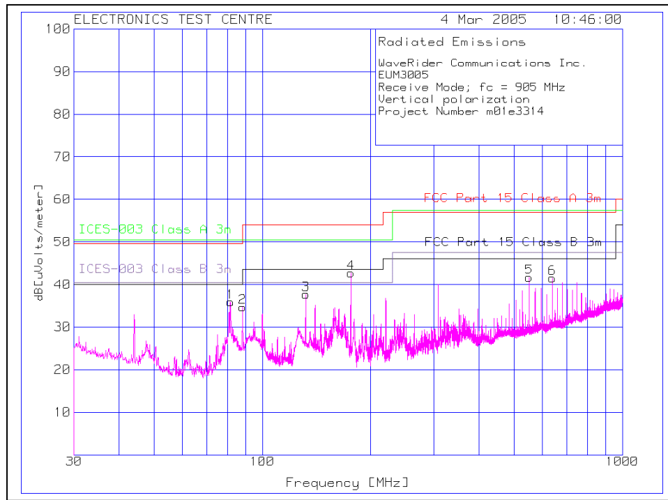
Plot of Radiated Emissions: Receive mode f_c = 905 MHz
