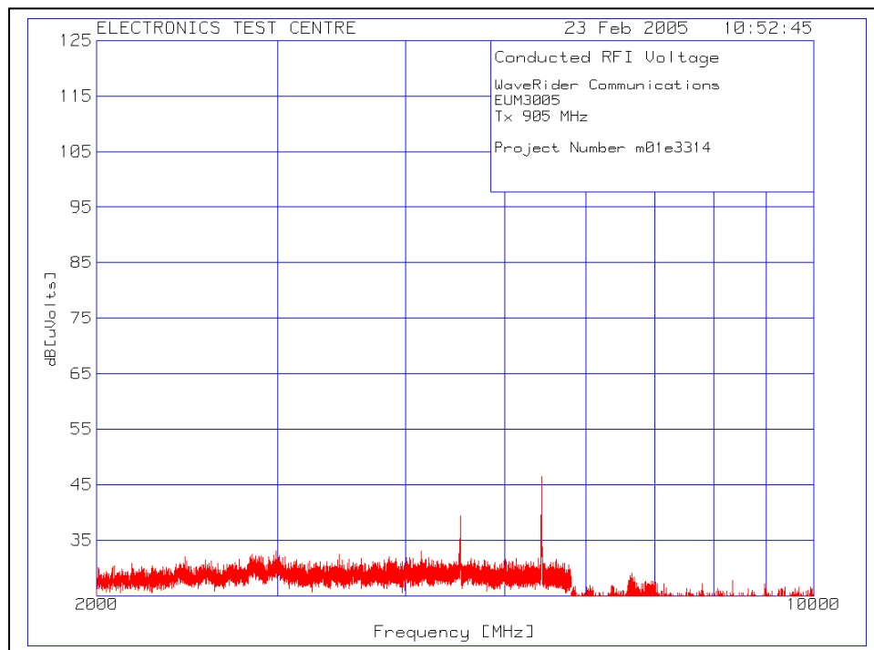
Plot of Conducted Emissions at Antenna Port: f_c = 905 MHz
