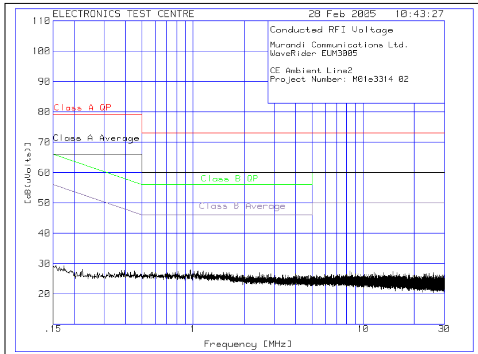
Plot of Conducted Emissions on AC Power Lines: Test Chamber ambient Line 2
