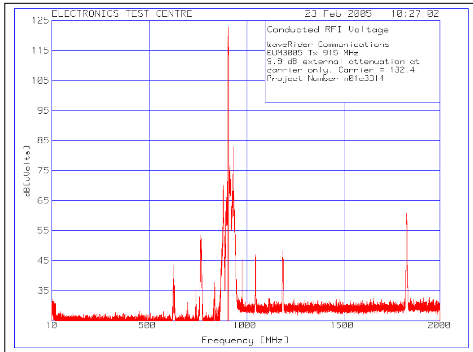
Plot of Conducted Emissions at Antenna Port: f_c = 915 MHz
