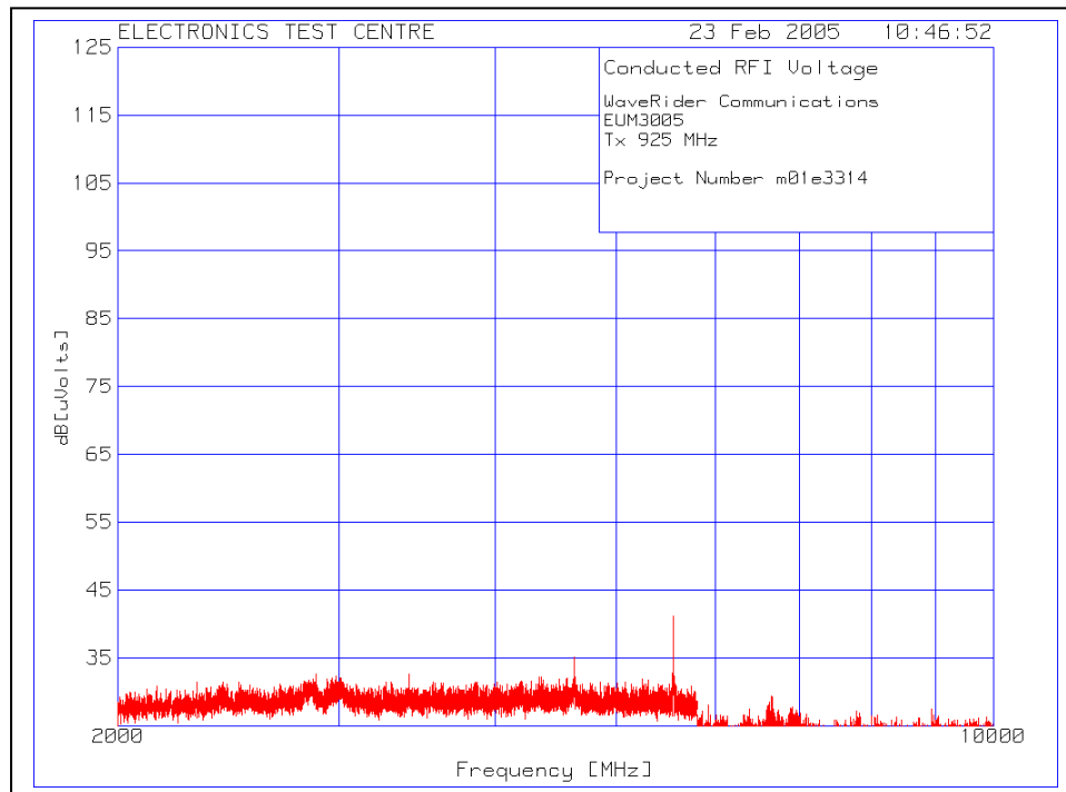
Plot of Conducted Emissions at Antenna Port: f_c = 925 MHz
