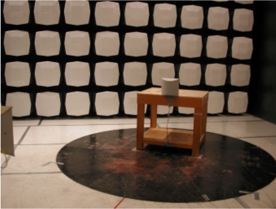
Transmit Radiated Emissions – Patch antenna
