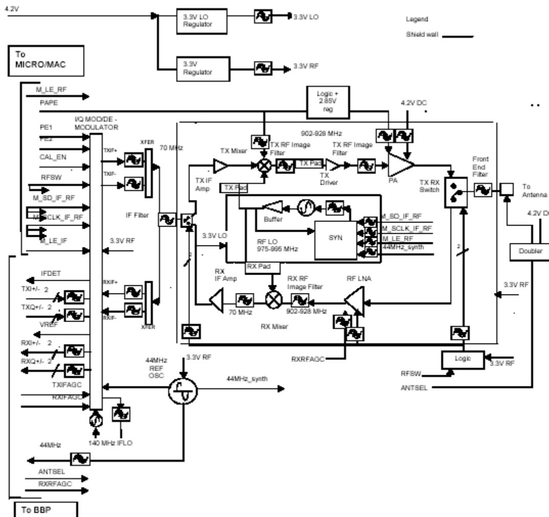
Figure 1.2 – RF Section Block Diagram
