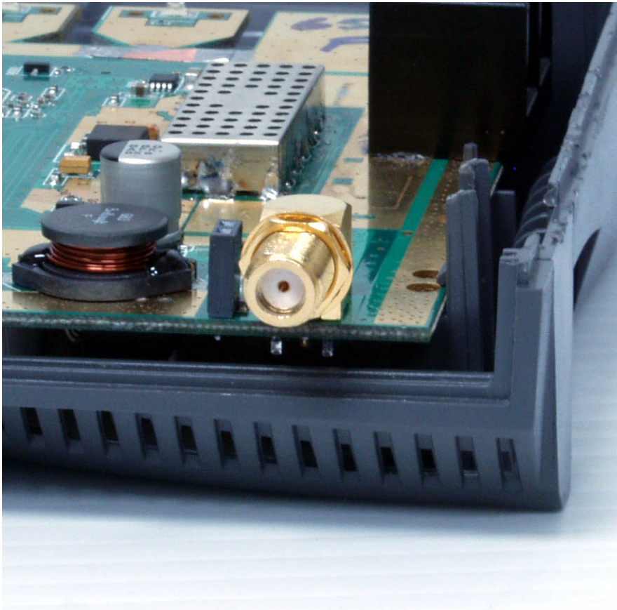
EUM8005 connector
