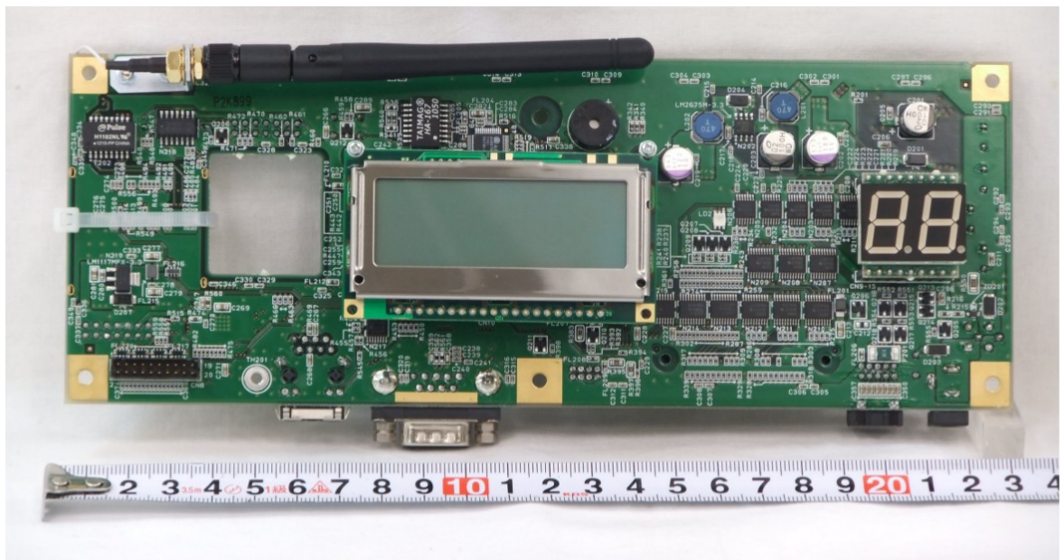
06-2: VPMAIN-C PKG Solder Side (with VPMAIN-LCD PKG)
