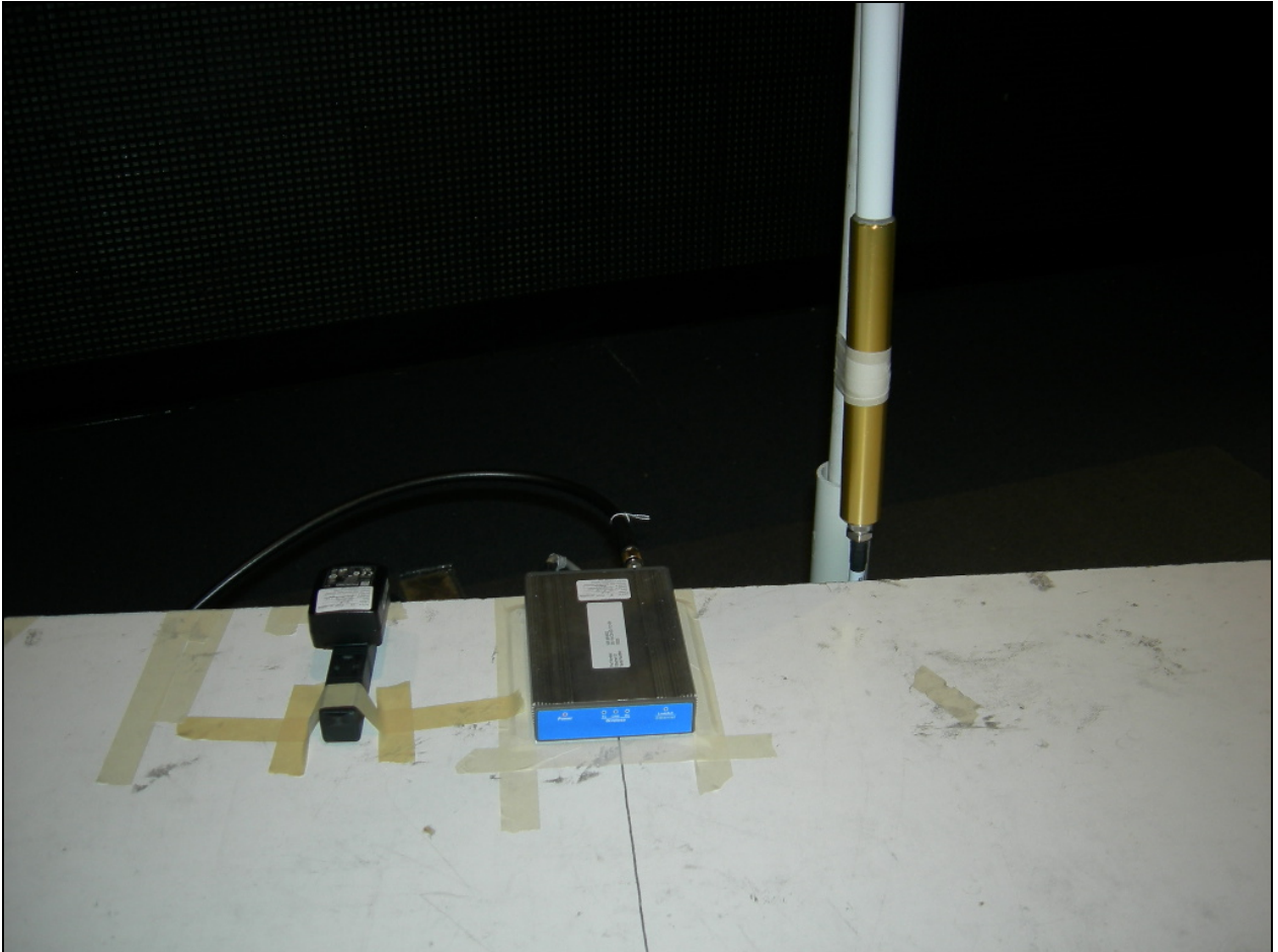
Figure 2: Radiated Emissions (Omni)
