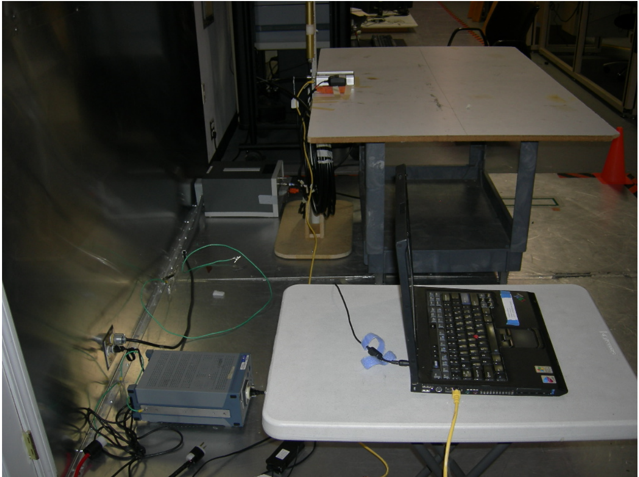
Figure 6: Conducted Emissions – (Omni)
