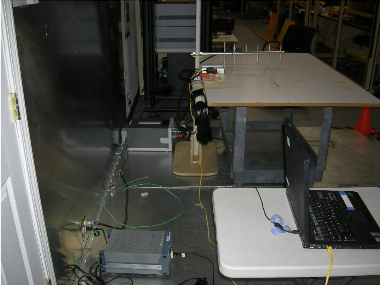
Figure 8: Conducted Emissions – (Yagi)
