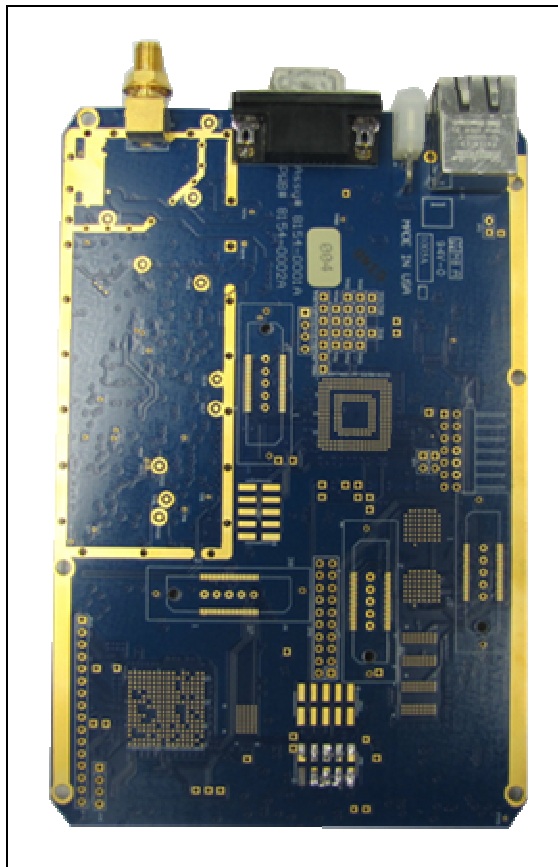
Figure 3: PCB - Back
