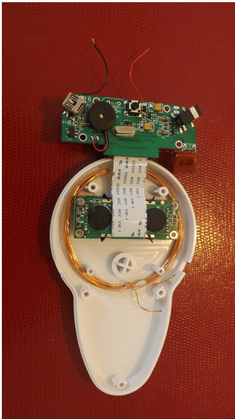
TOP BOARD BACK VIEW
