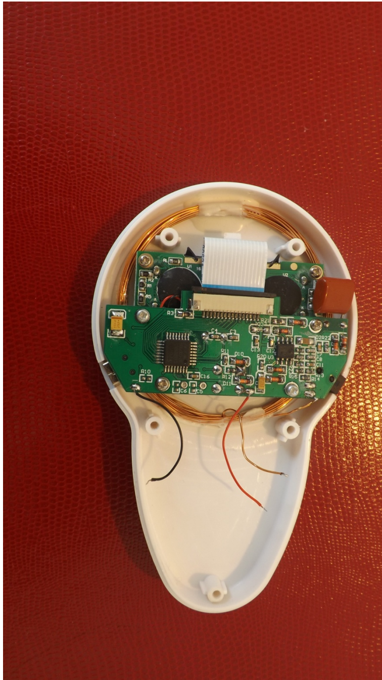
INTERNAL PHOTO COVER OFF – TWO BOARDS IN READER
