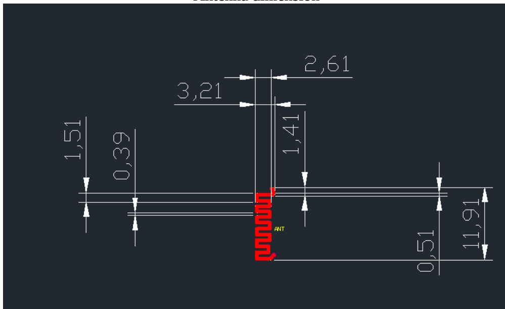
Antenna dimension
