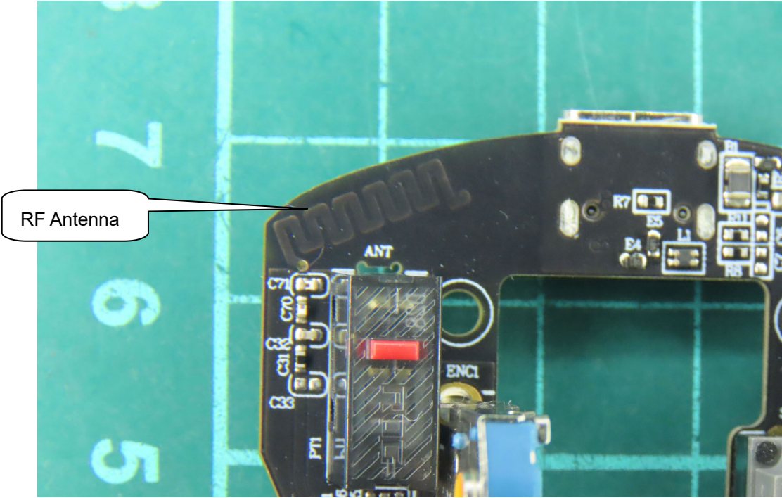
(24)EUT Photo
