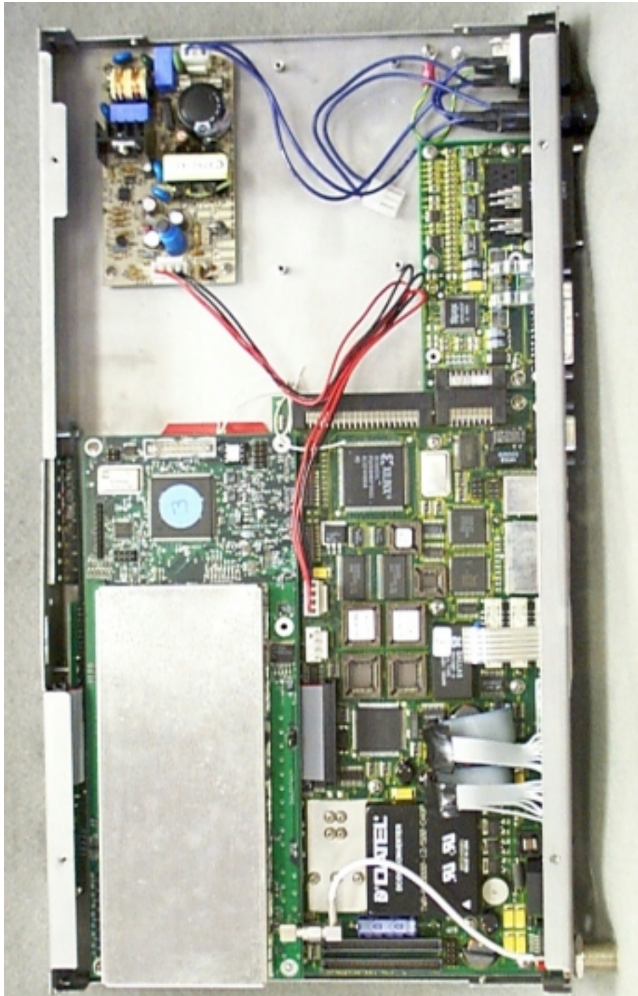
Photo 4. EUT, Top View (Cover Removed)
