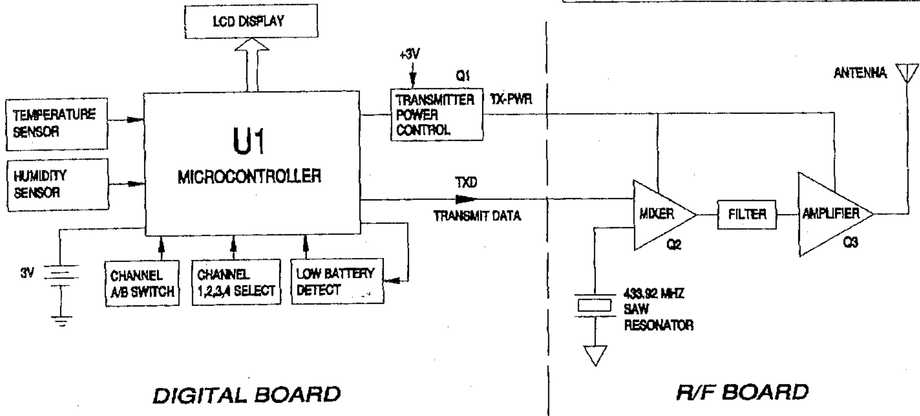
BLOCK DIAGRAM OF RFTH RX TRANSMITTER
