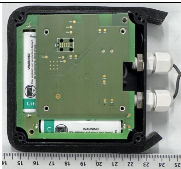
PCB rear view (main board)
