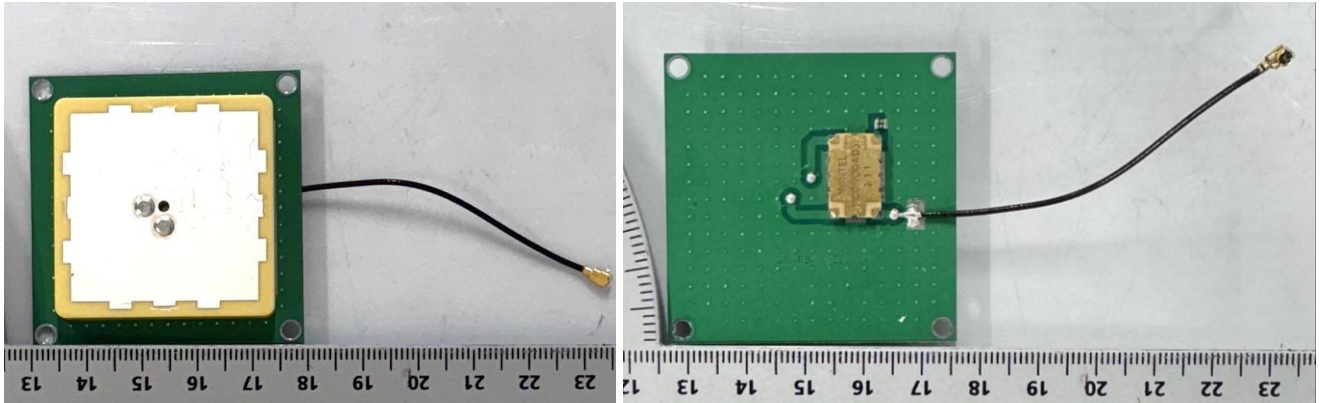
UHF Antenna
