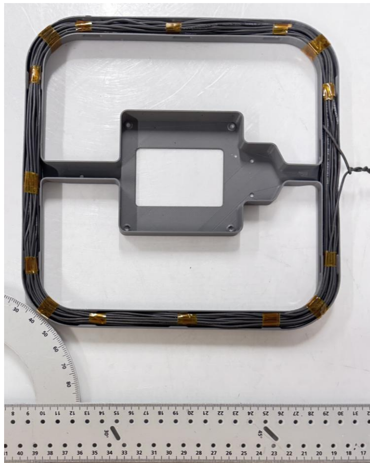
LF Antenna
