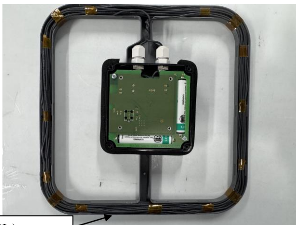
LF (125kHz) antenna
