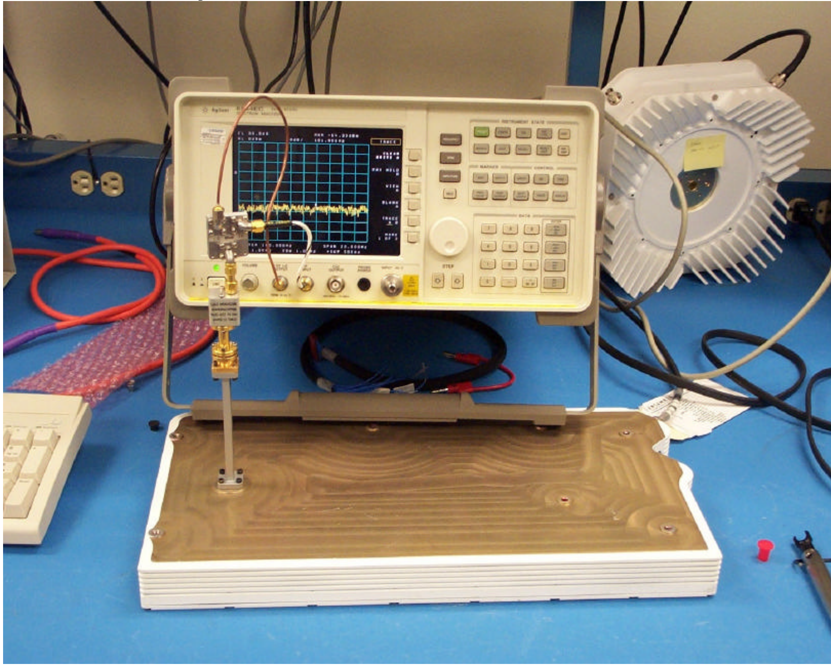
Base Station ODU Test Set Up for 40 GHz-200 GHz
