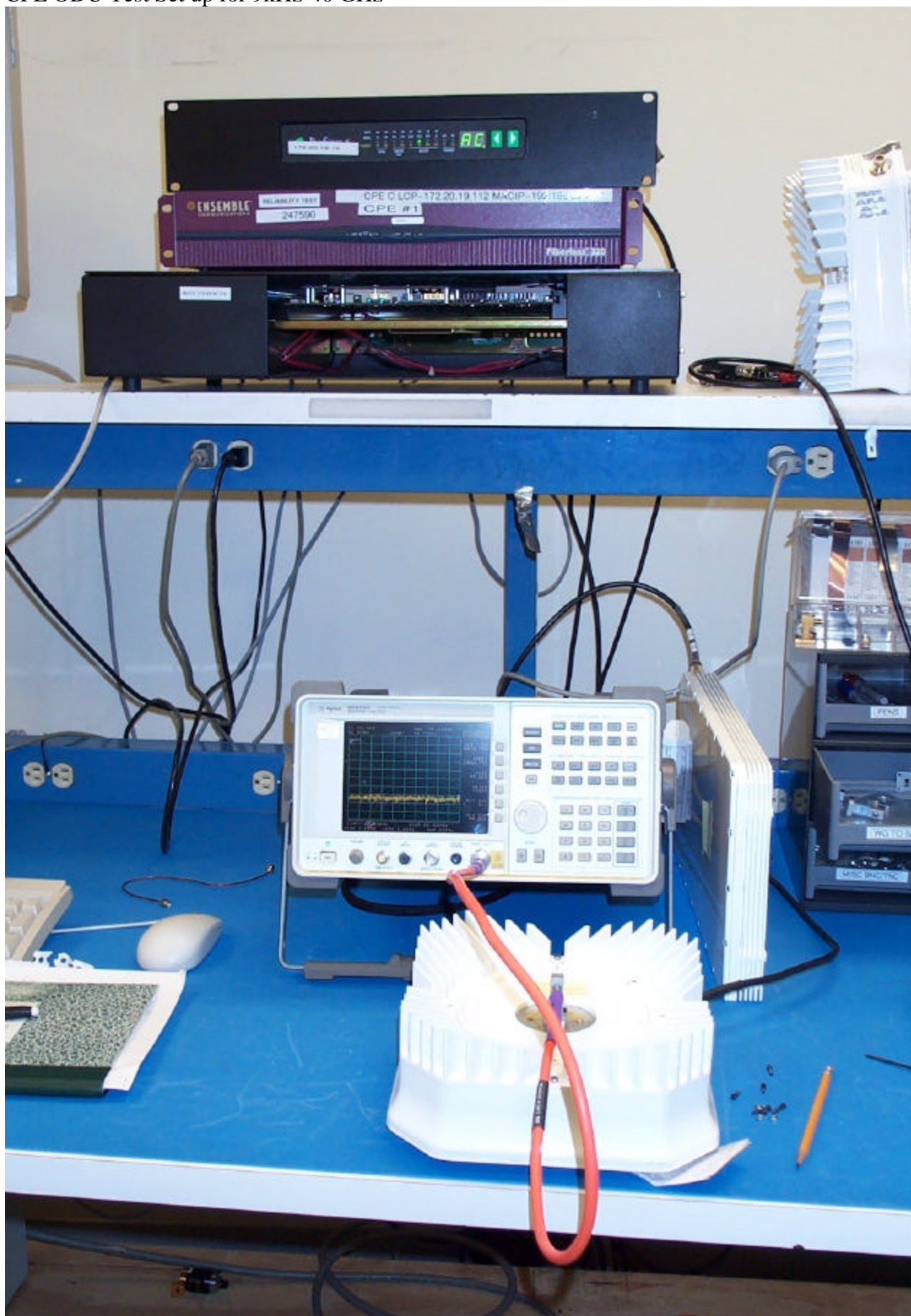
CPE ODU Test Set up for 9kHz-40 GHz
