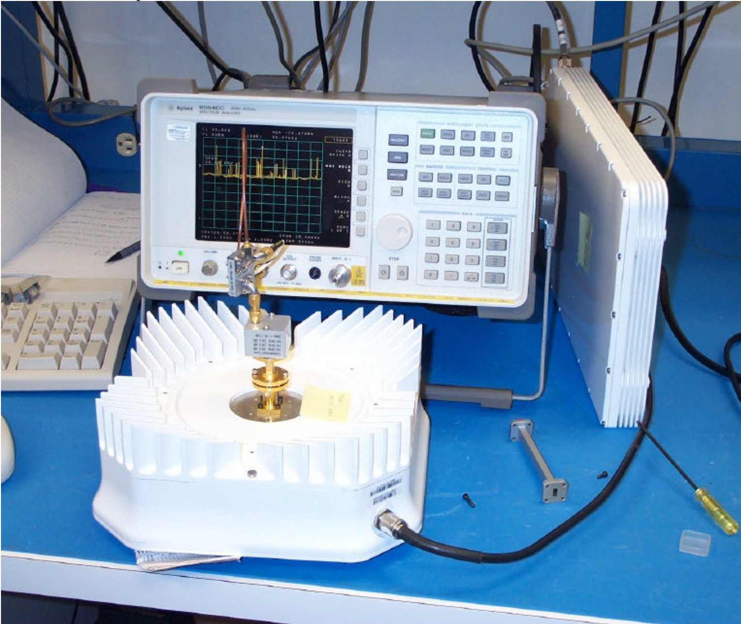
CPE ODU Test Set Up 40 GHz - 200 GHz
