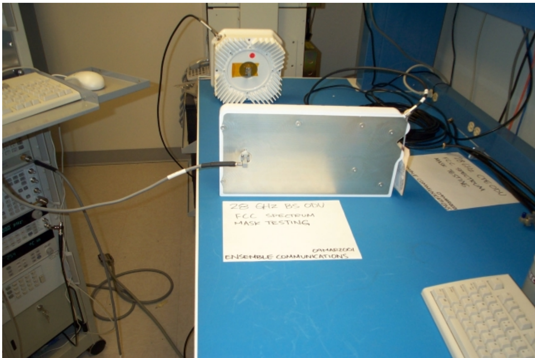
BS-ODU Test Hook-up
