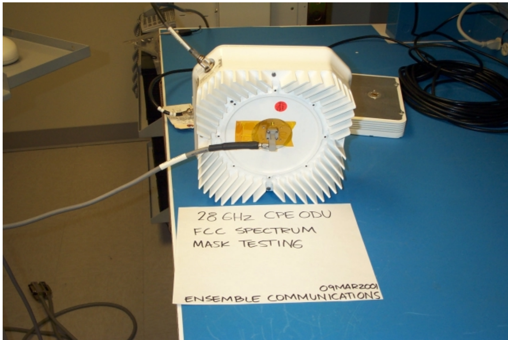
CPE-ODU Test Hook-up
