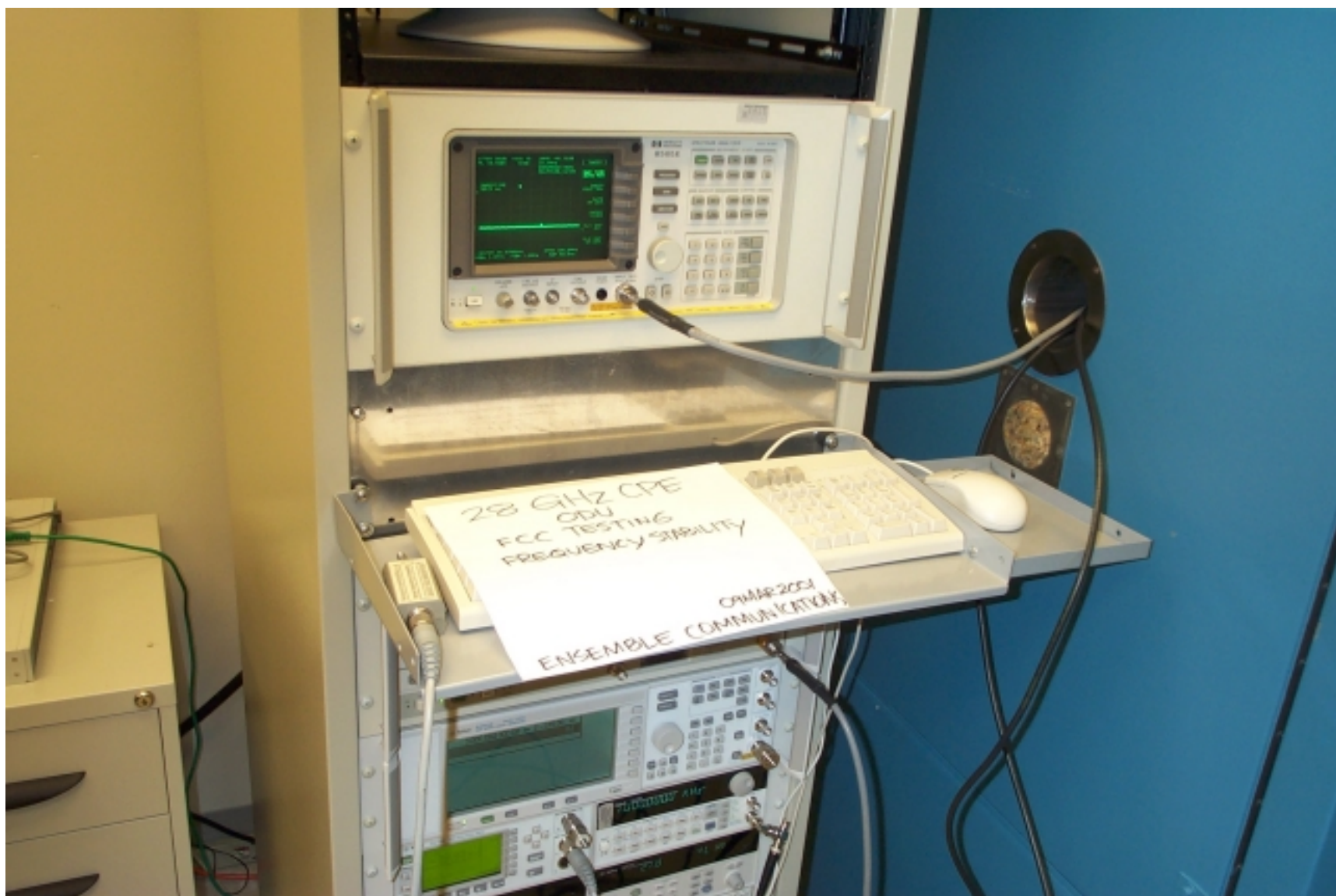
Spectrum Analyzer Cabling into Temperature Chamber
