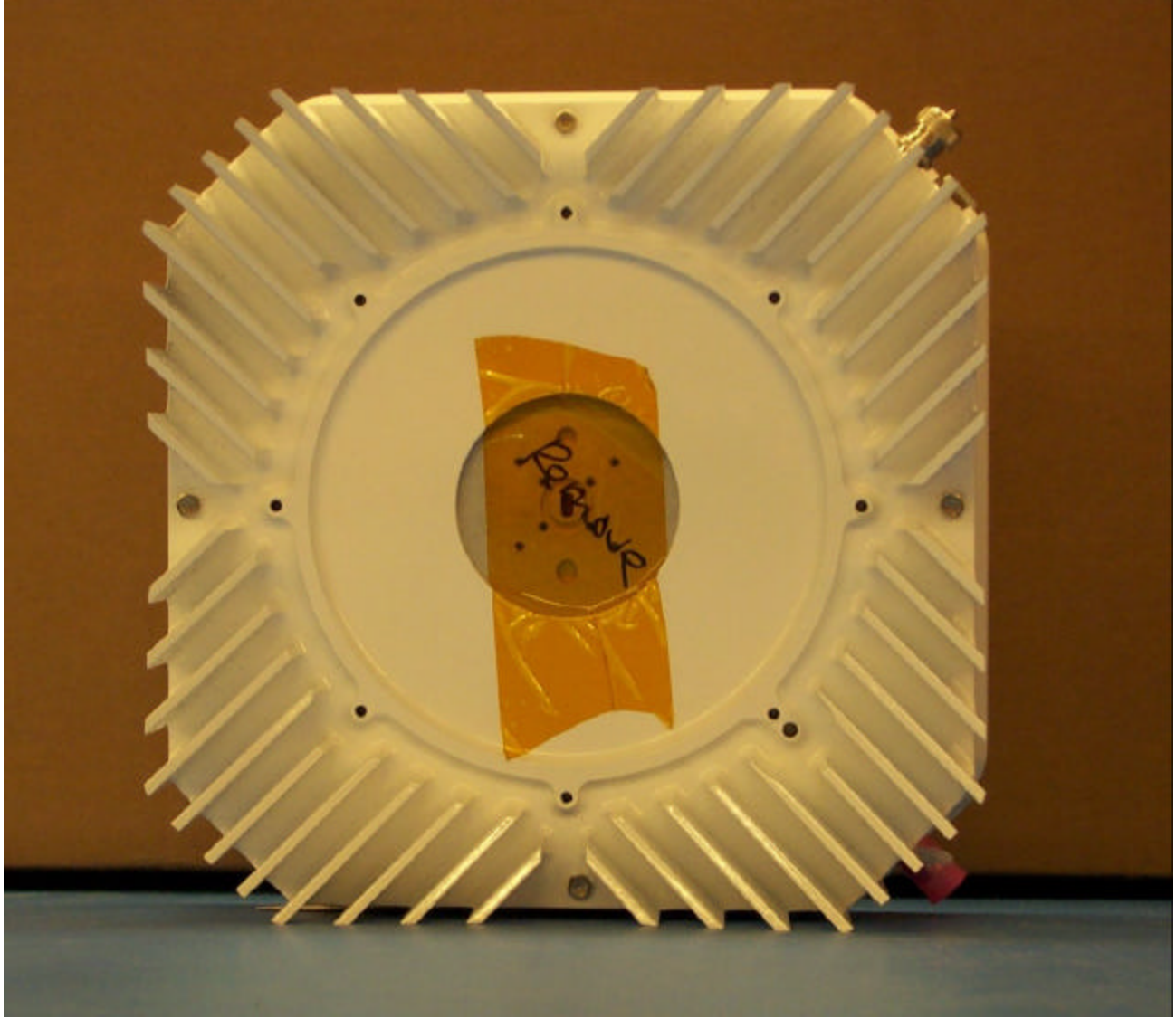
CPE ODU, no antenna Front view
