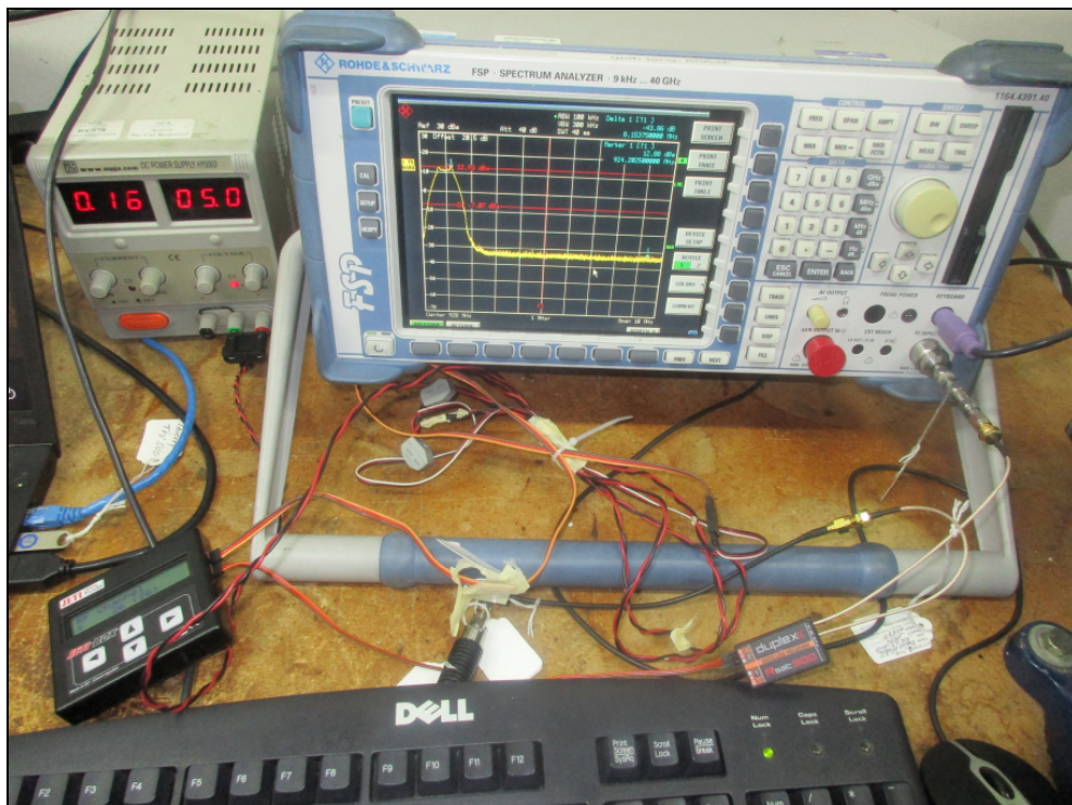
Figure 6: RF Conducted
