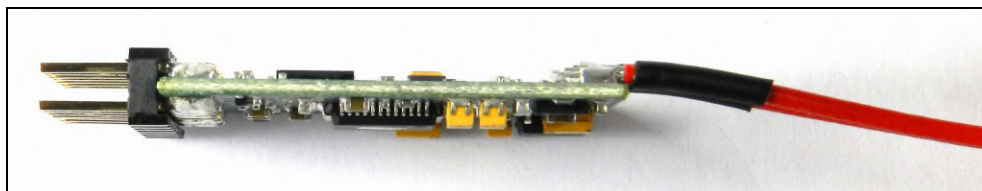
Figure 3: PCB Front
