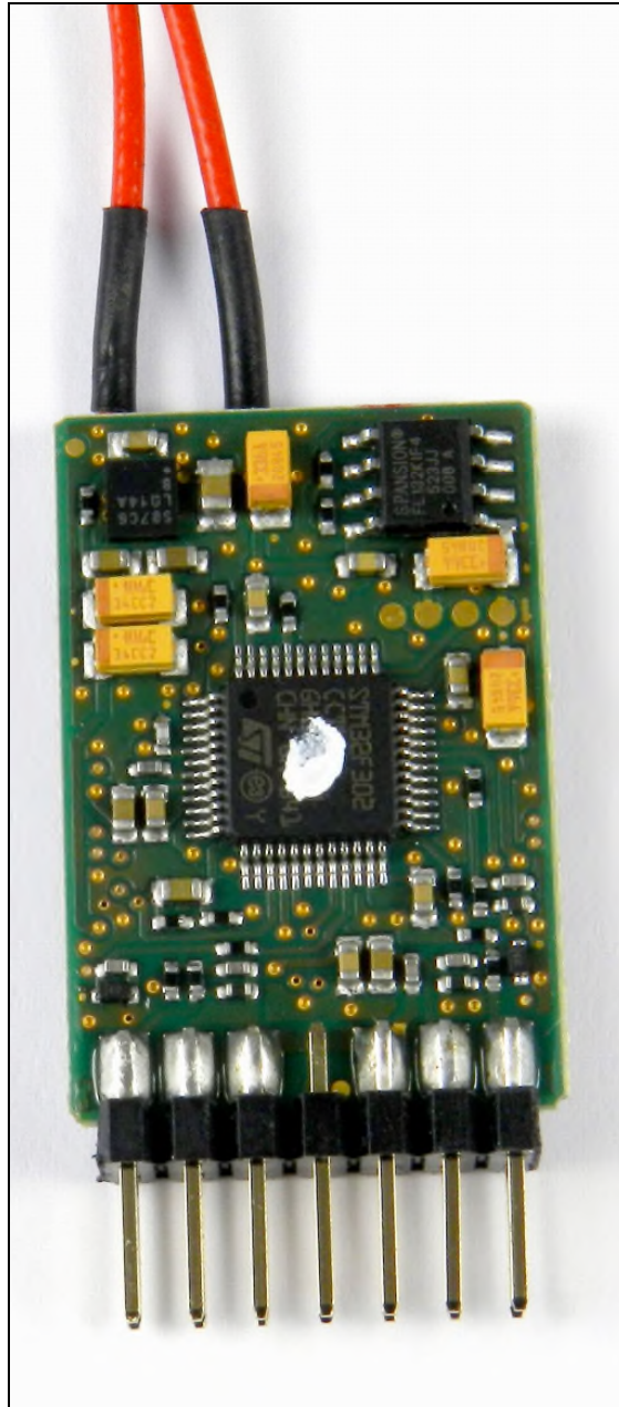
Figure 2: PCB Bottom
