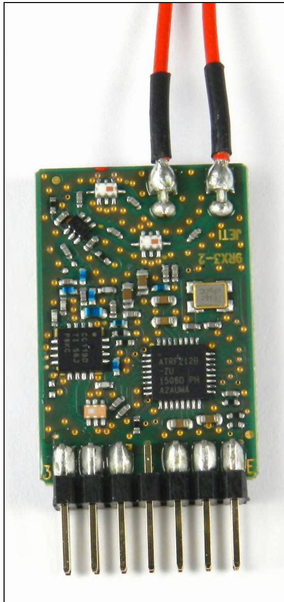
Figure 1: PCB Top
