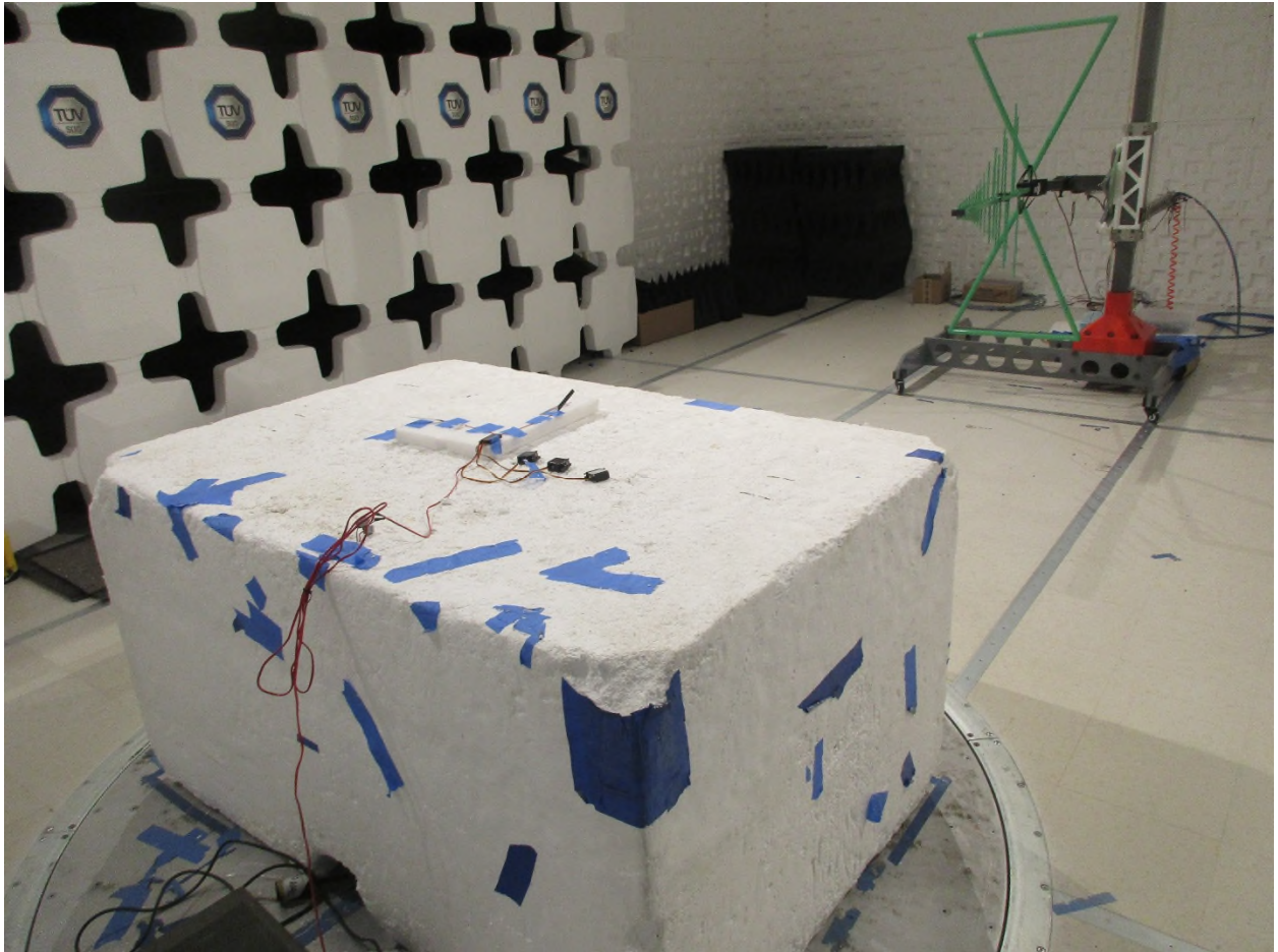
Figure 3: Radiated Emissions – Back View – 30 MHz to1 GHz
