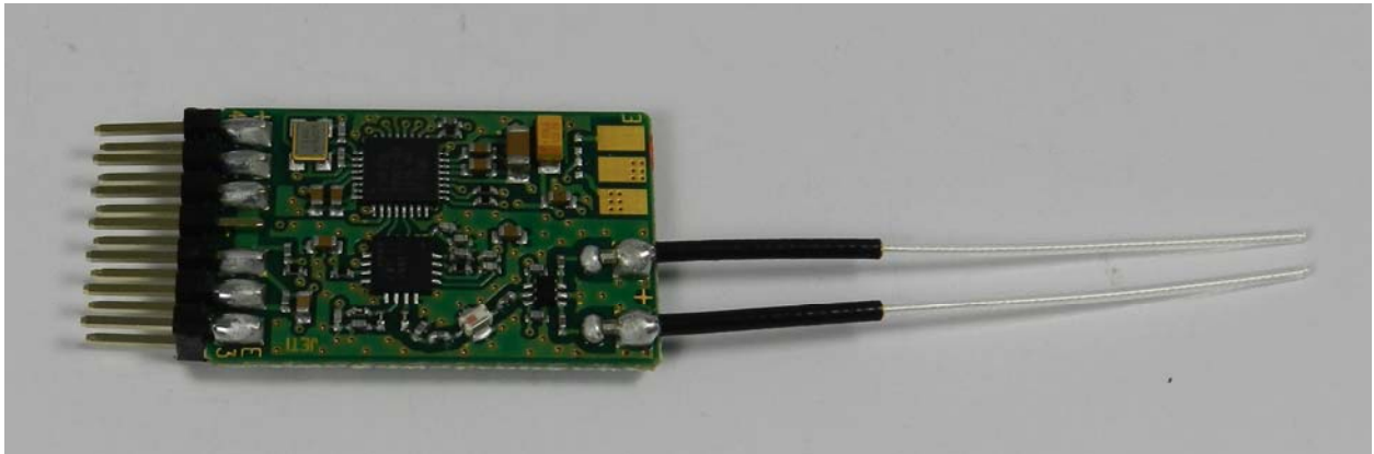
Figure 7: JETIR4iUS (PCB Top View)
