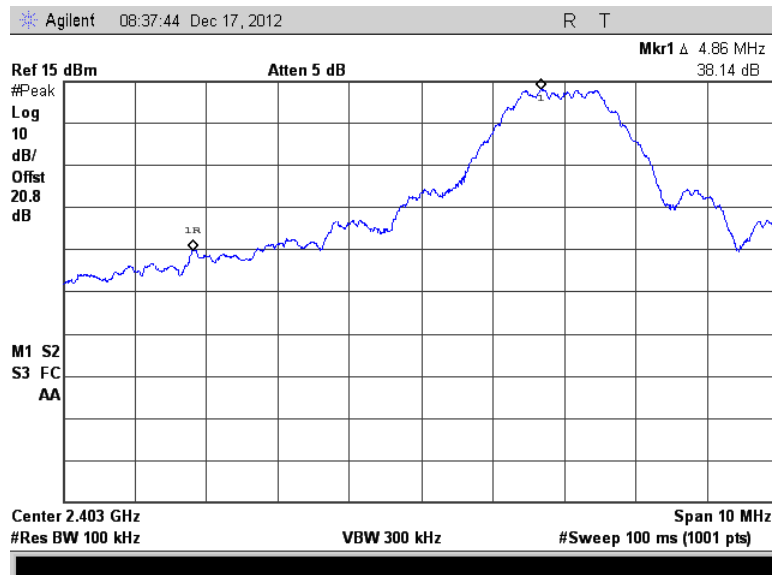
Figure 7.4.1.2-1: Lower Band-edge – 2405 MHz
