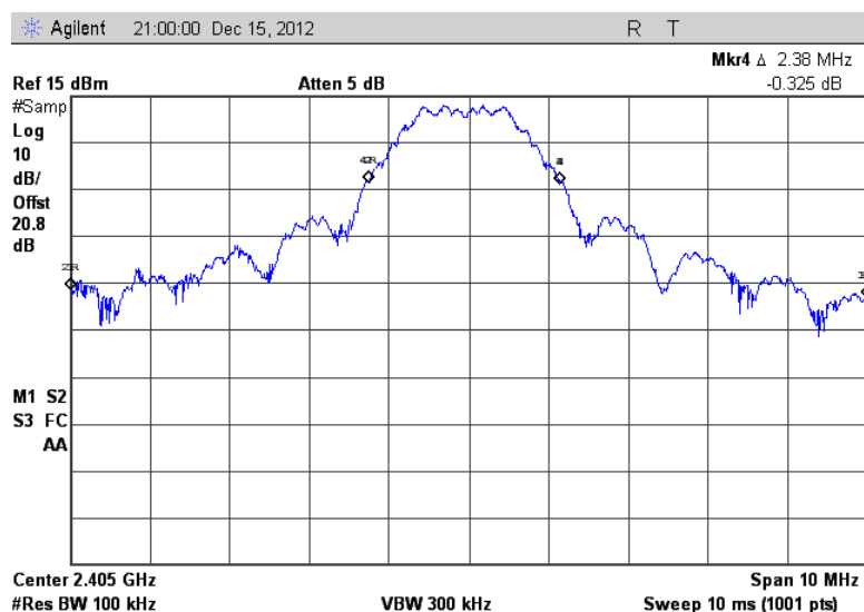
Figure 7.3.4.2-10: 99% OBW Low Channel
