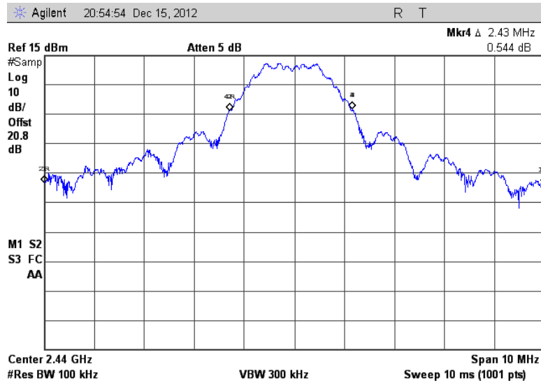
Figure 7.3.4.2-11: 99% OBW Middle Channel
