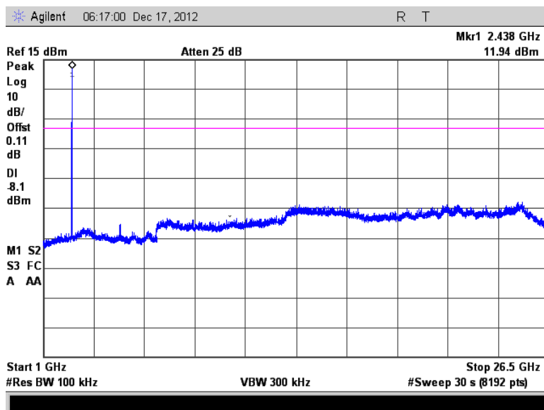
Figure 7.4.2.2-10: 1 GHz –26.5 GHz – Middle Channel
