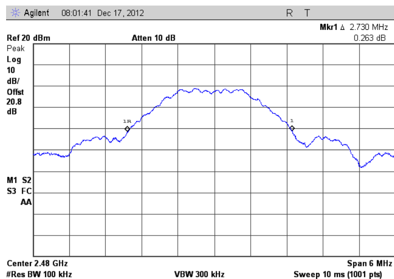
Figure 7.3.4.2-3: 20dB BW High Channel
