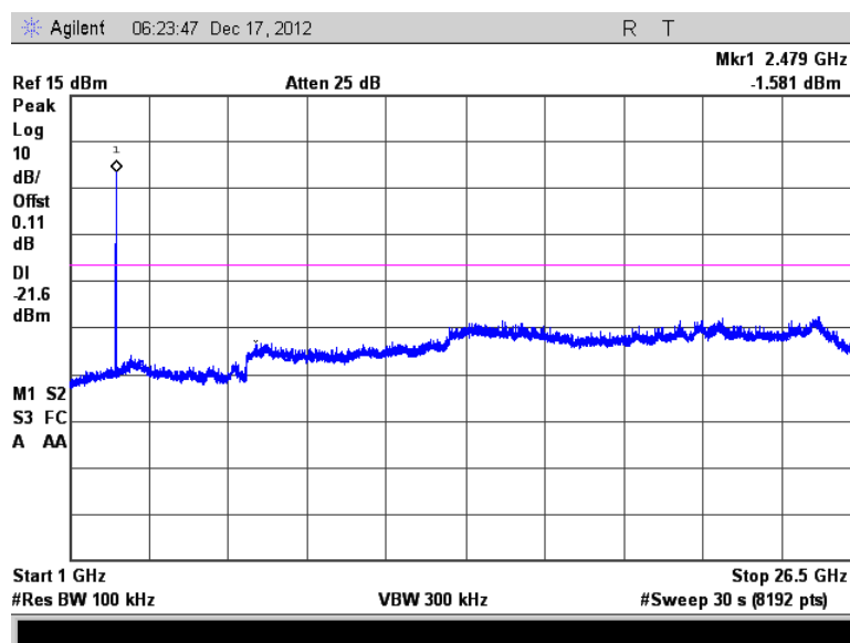
Figure 7.4.2.2-12: 1 GHz –26.5 GHz – High Channel
