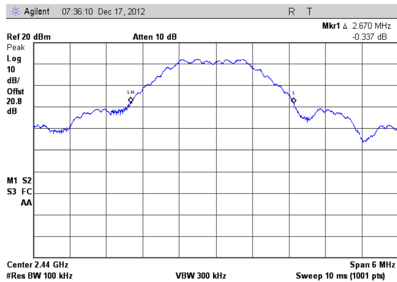
Figure 7.3.4.2-2: 20dB BW Middle Channel
