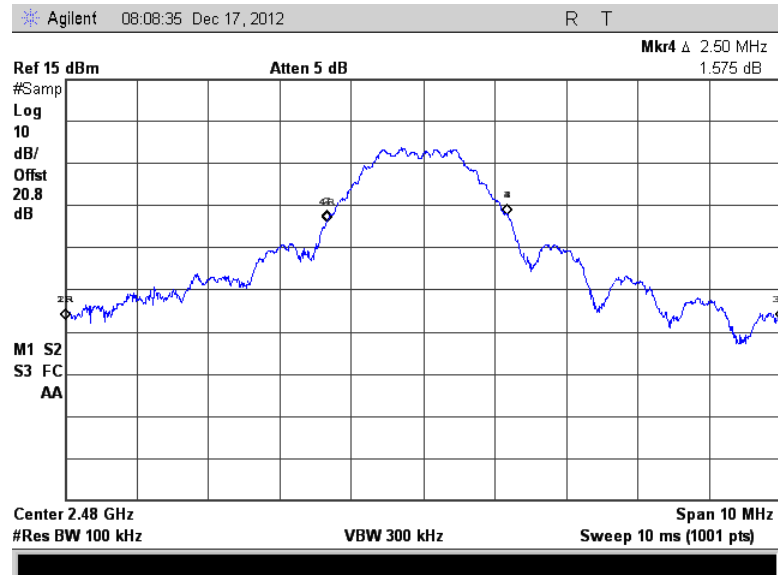
Figure 7.3.4.2-6: 99% OBW High Channel
