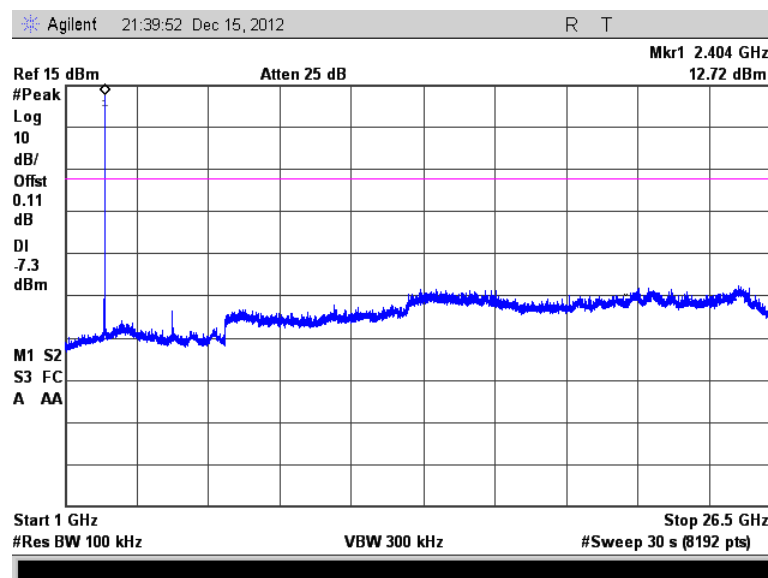
Figure 7.4.2.2-8: 1 GHz –26.5 GHz – Low Channel
