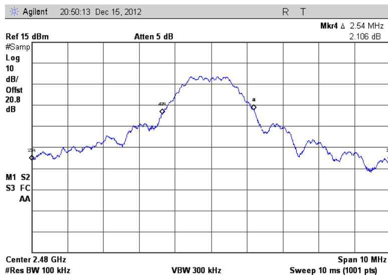
Figure 7.3.4.2-12: 99% OBW High Channel
