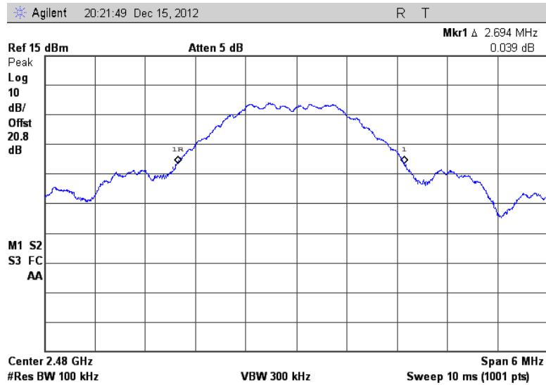
Figure 7.3.4.2-9: 20dB BW High Channel
