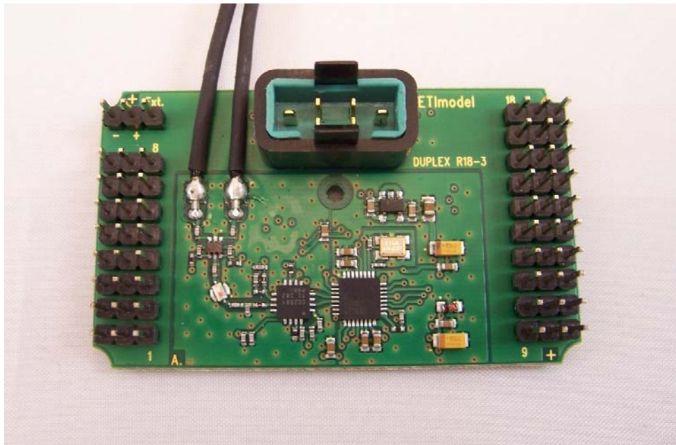
Figure 4: JETIR14US (PCB Bottom View)
