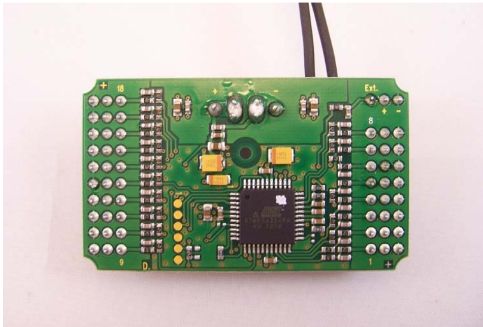
Figure 1: JETIR18US (PCB Top View)
