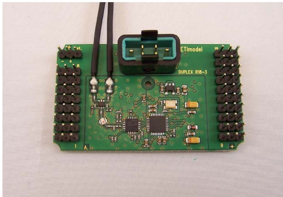
Figure 2: JETIR18US (PCB Bottom View)
