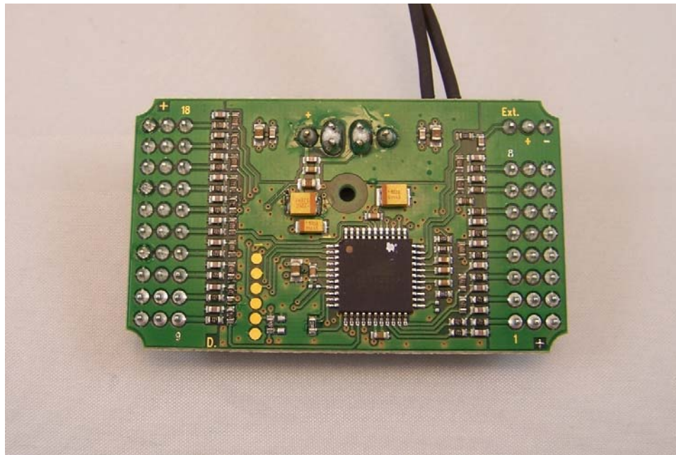
Figure 3: JETIR14US (PCB Top View)
