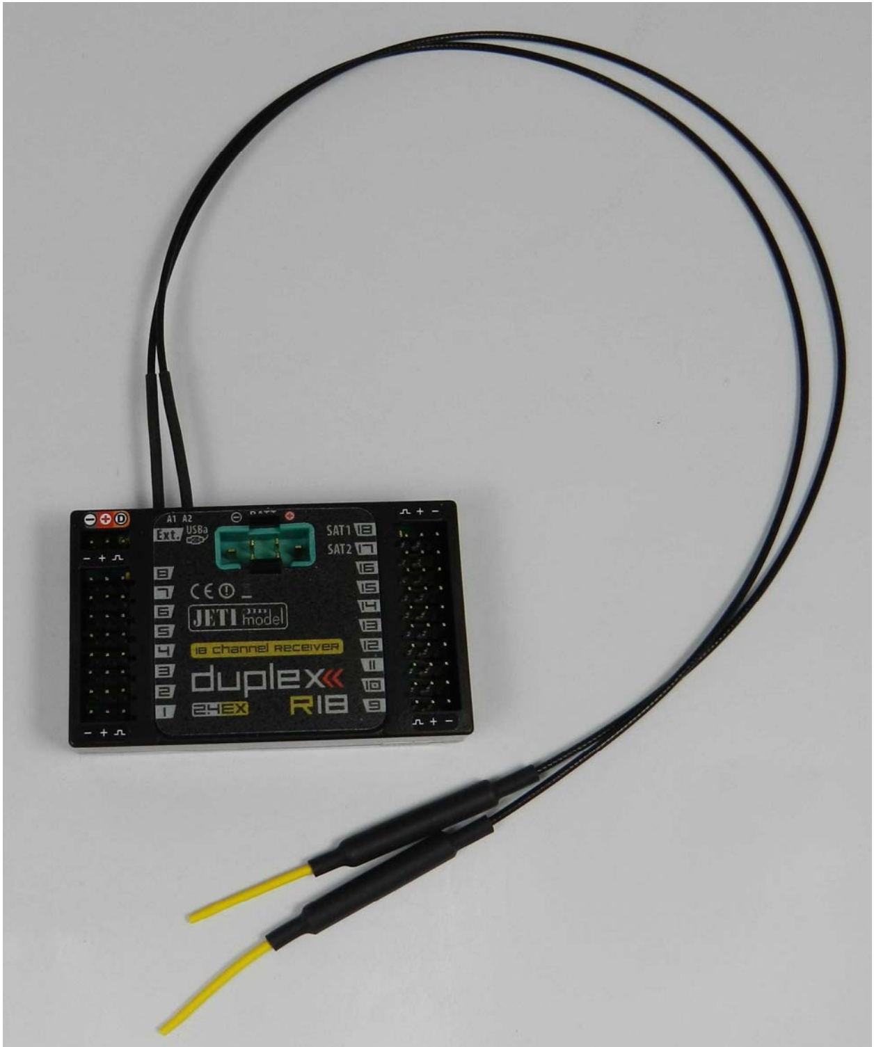
Figure 1: JETIR18US (Top View)
