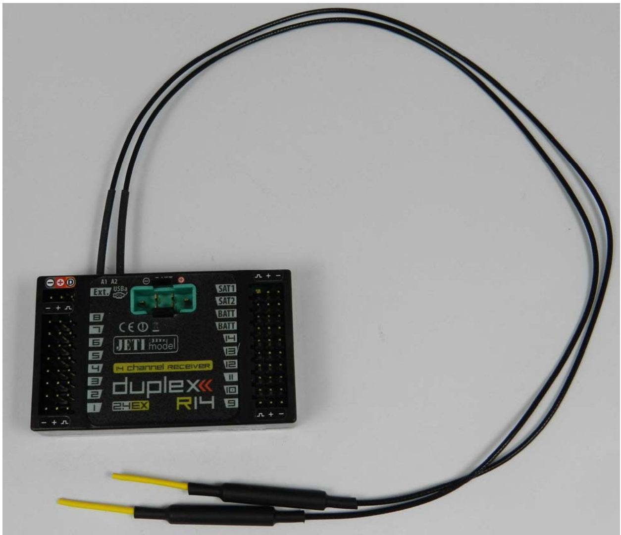
Figure 7: JETIR14US (Top View)
