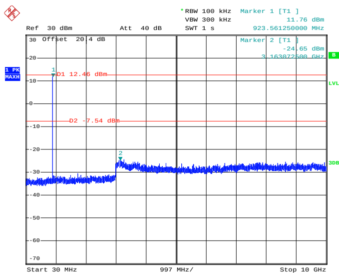
Figure 7.4.2.2-2: 30 MHz – 10 GHz – Middle Channel
