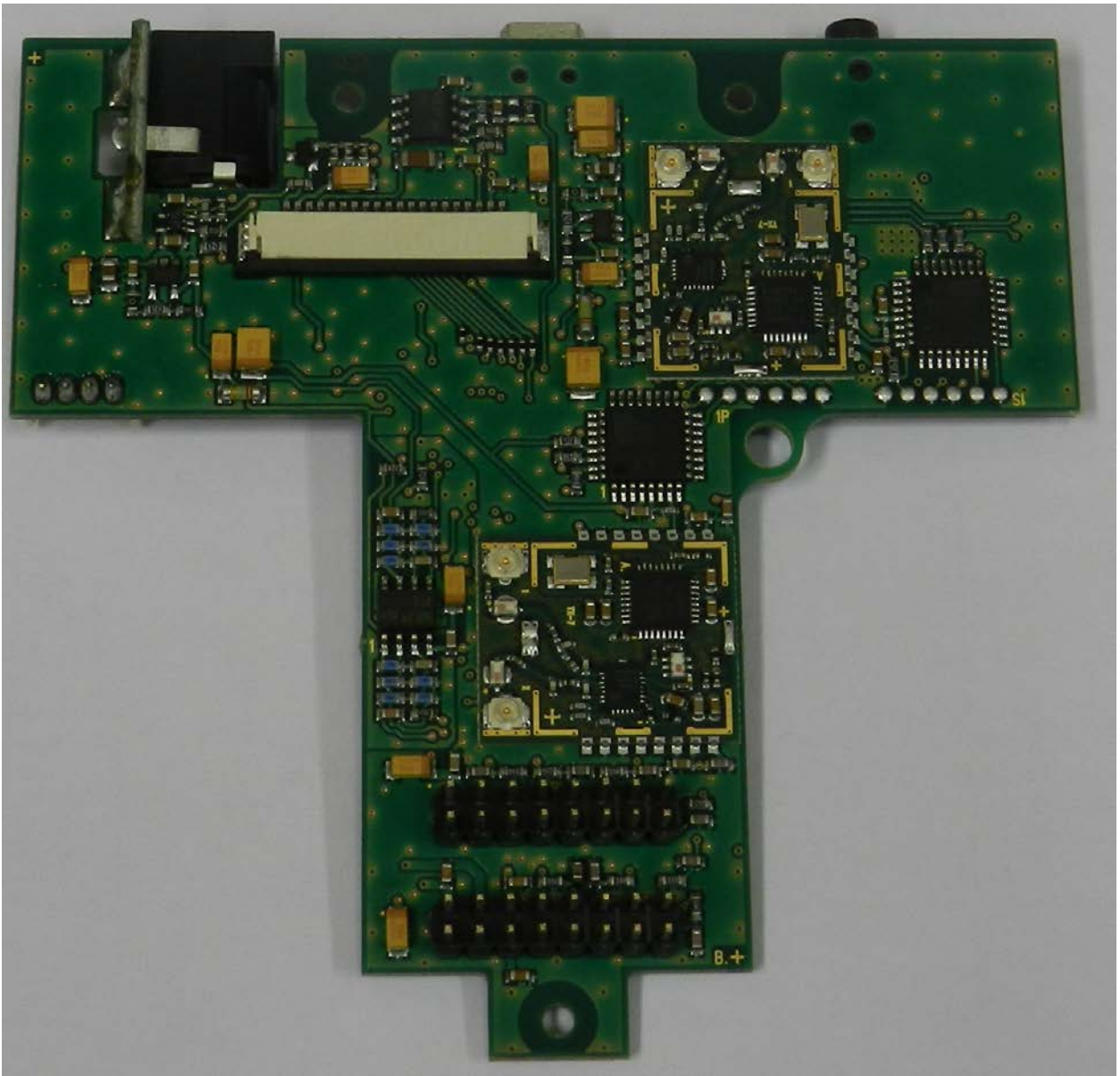
Figure 4: DS-CONT-2 Board Bottom (without Shield)
