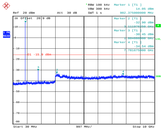
Figure 2.9.6-3: Conducted Spurious Emissions – High Channel – SF6
