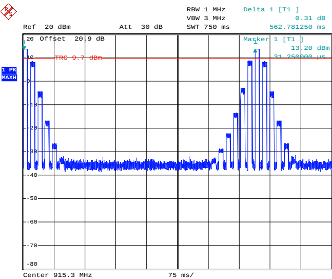
Figure 2.4.6-1: Channel Dwell Time Test Results – SF6
