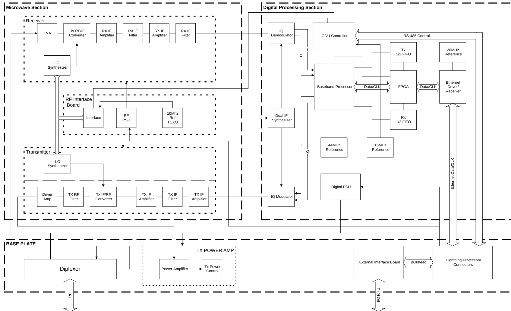
FIGURE 3: Radio Station Outdoor Unit Block Diagram and Interfaces
