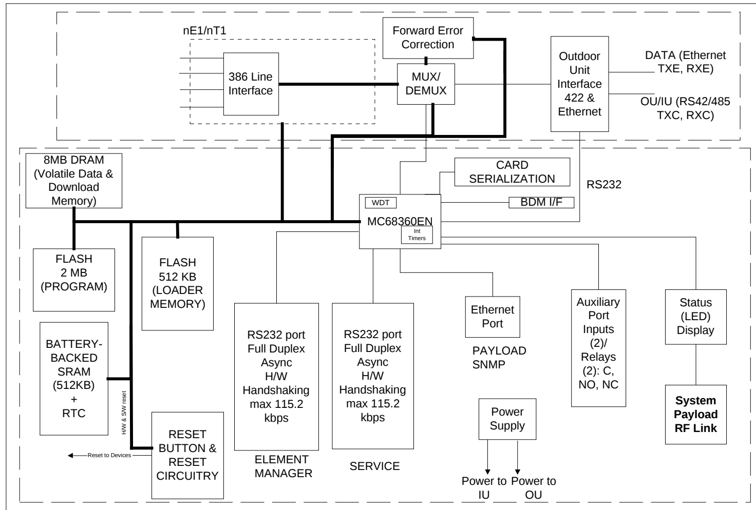
FIGURE 2: Radio Station Indoor Unit Block Diagram and Interfaces
