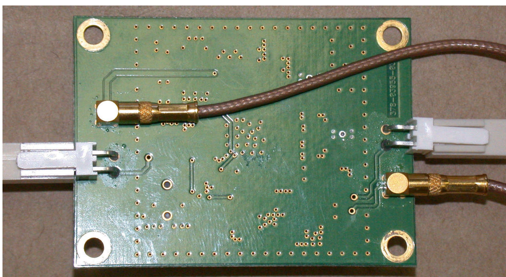
Spectrum Analyser PCB – top and bottom
