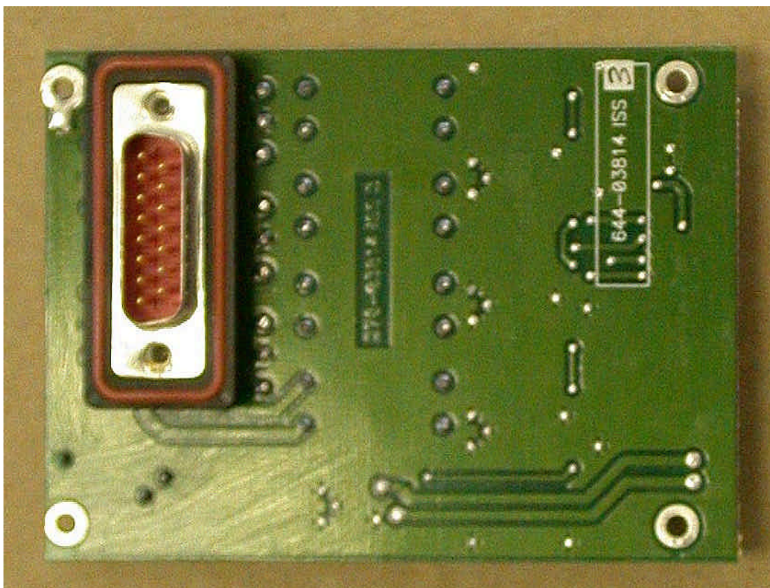
Lightning Protection PCB
