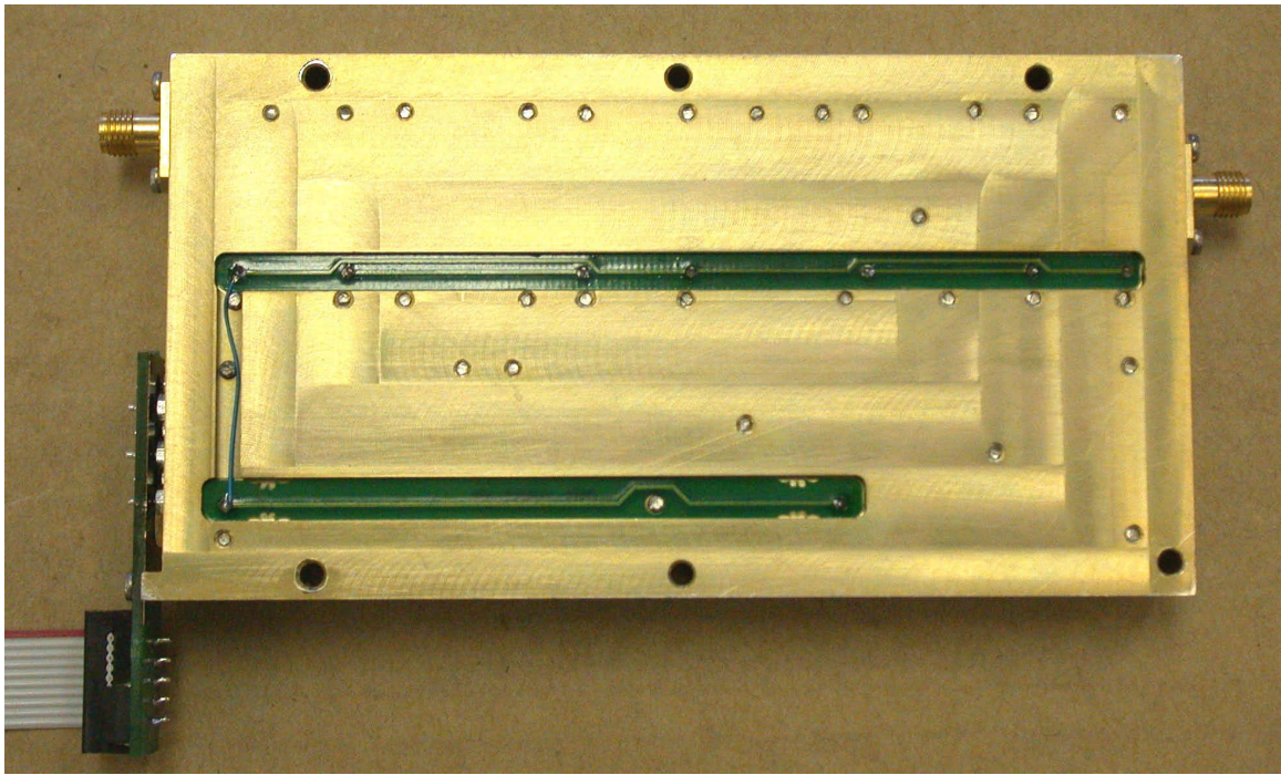
Tx Housing Bottom View
