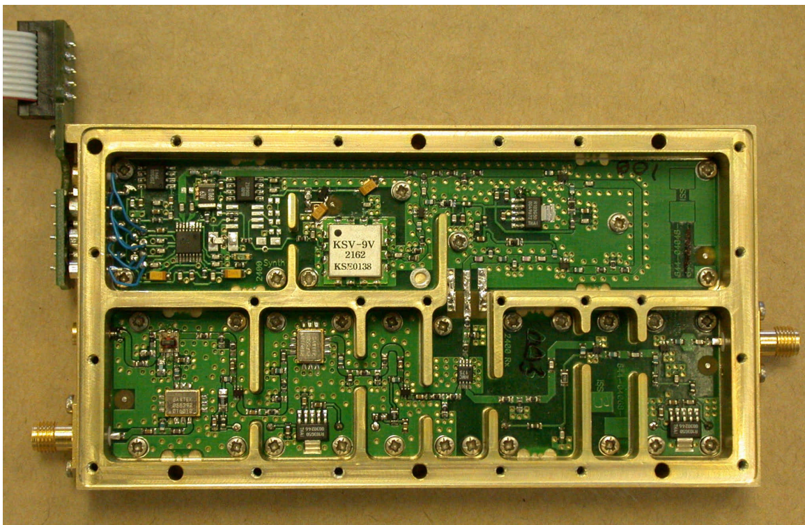
Rx Housing with Lid Removed
