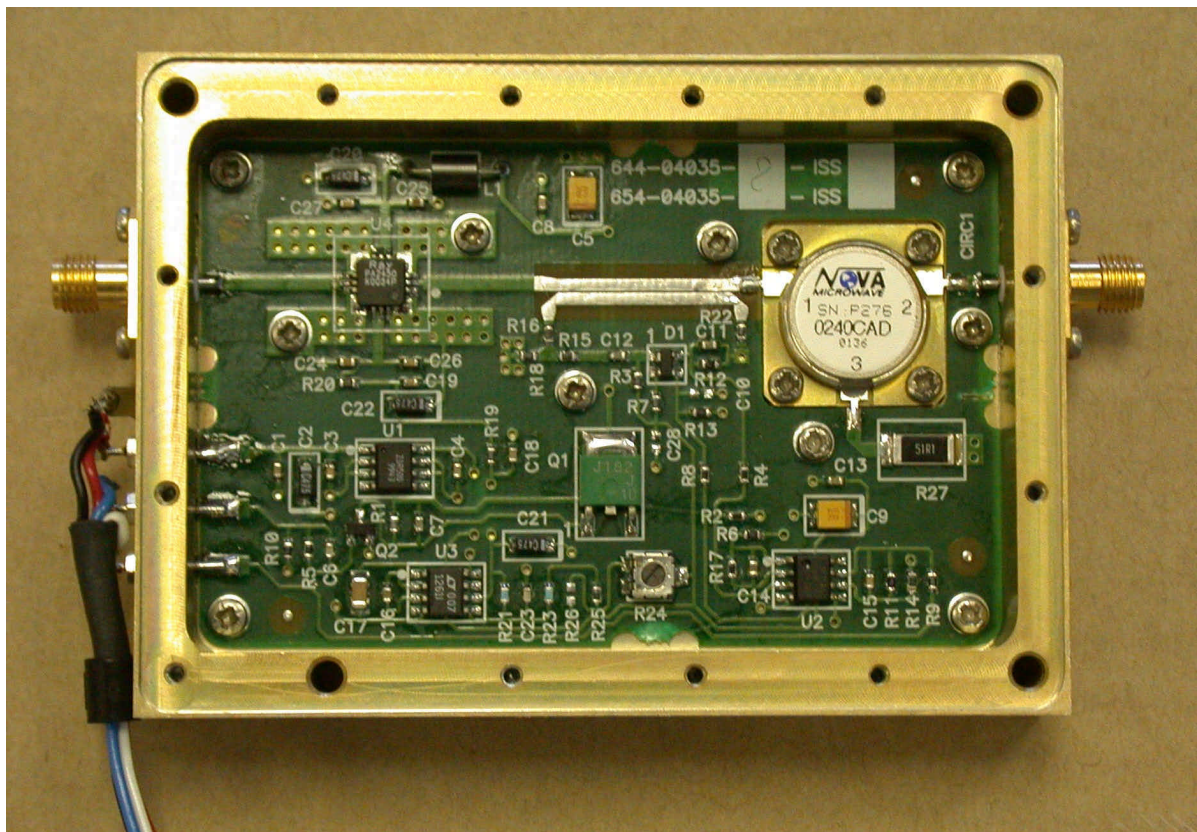
Power Amplifier with Lid Removed
