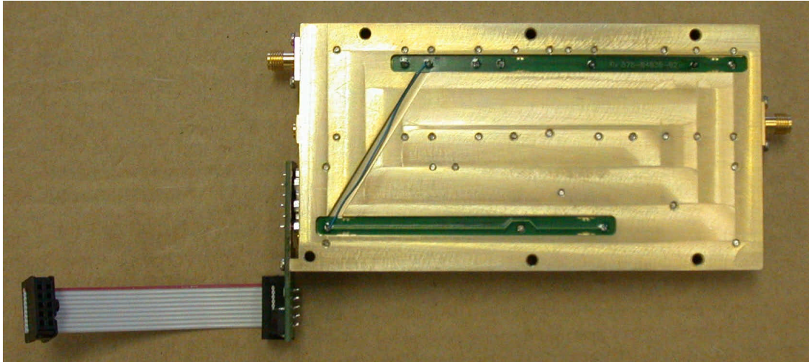
Rx Housing Bottom View
