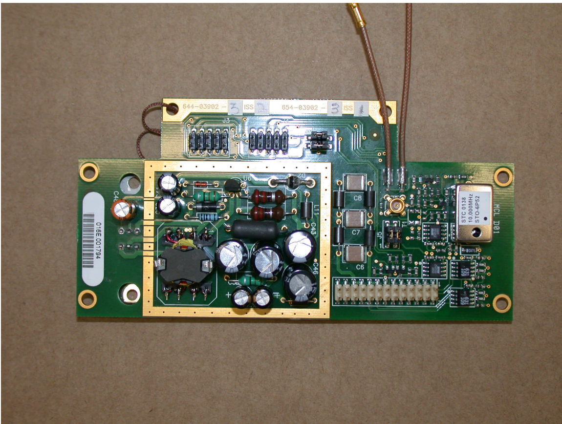
PSU/TCXO Top Assembly without Screening Can
