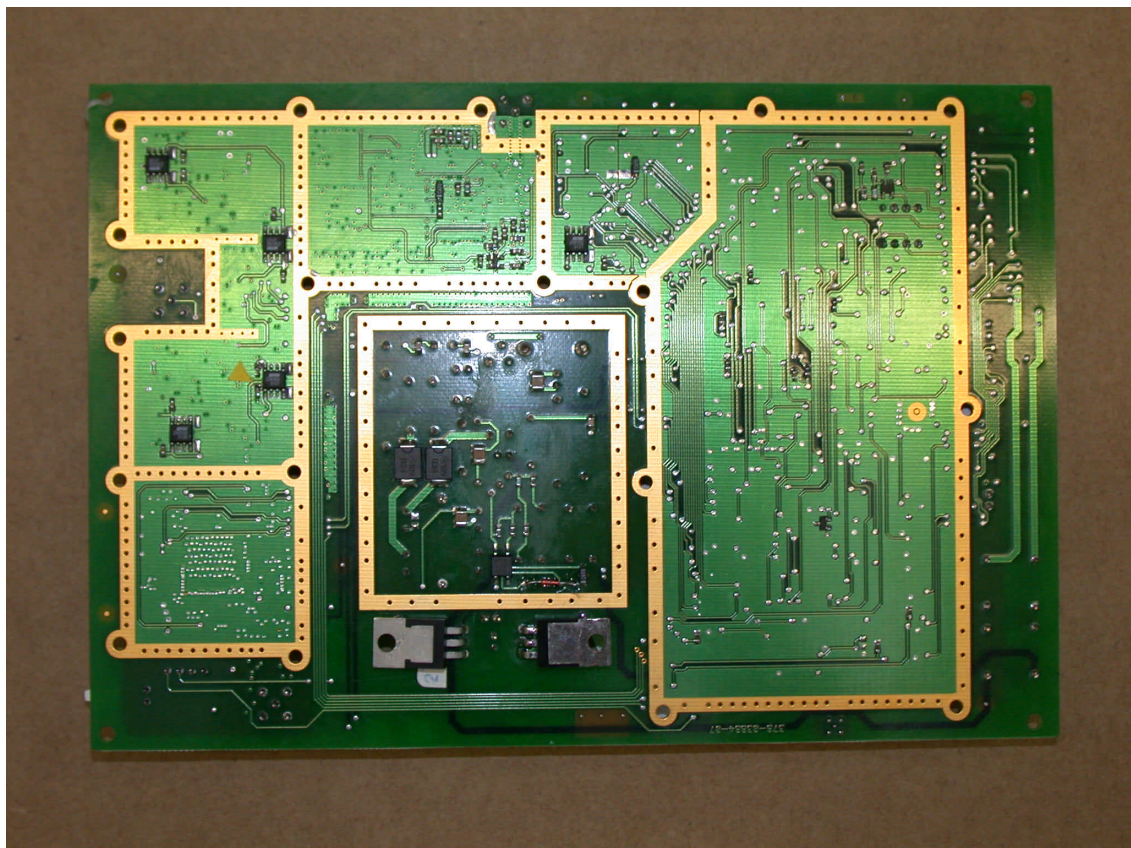
Baseband Processor PCB Bottom without Screening Can
