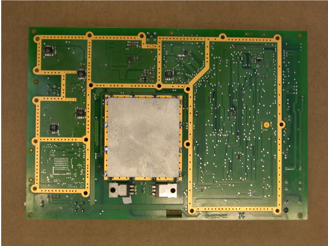
Baseband Processor PCB Bottom with Screening Can
