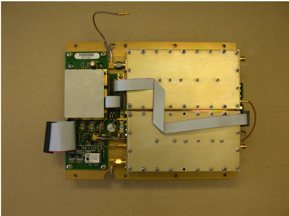
Baseband Processor Top Assembly with Cans
