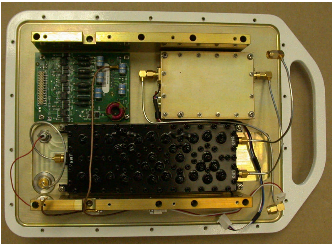
Outdoor Unit with no Baseband Processor Assembly
