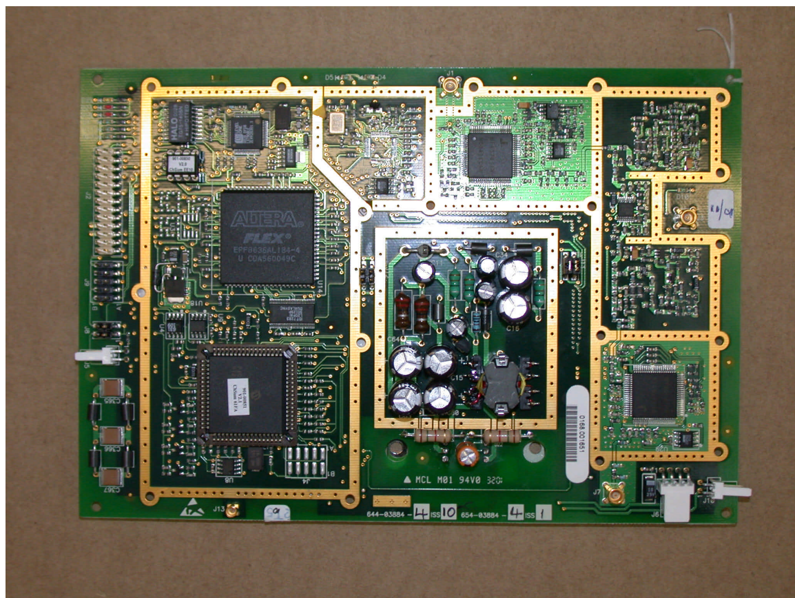
Baseband Processor PCB Top with Screening Can
