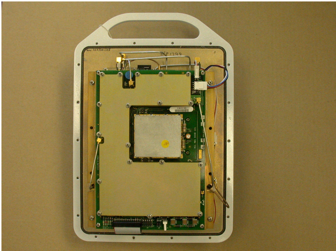
Outdoor Unit without Front Cover
