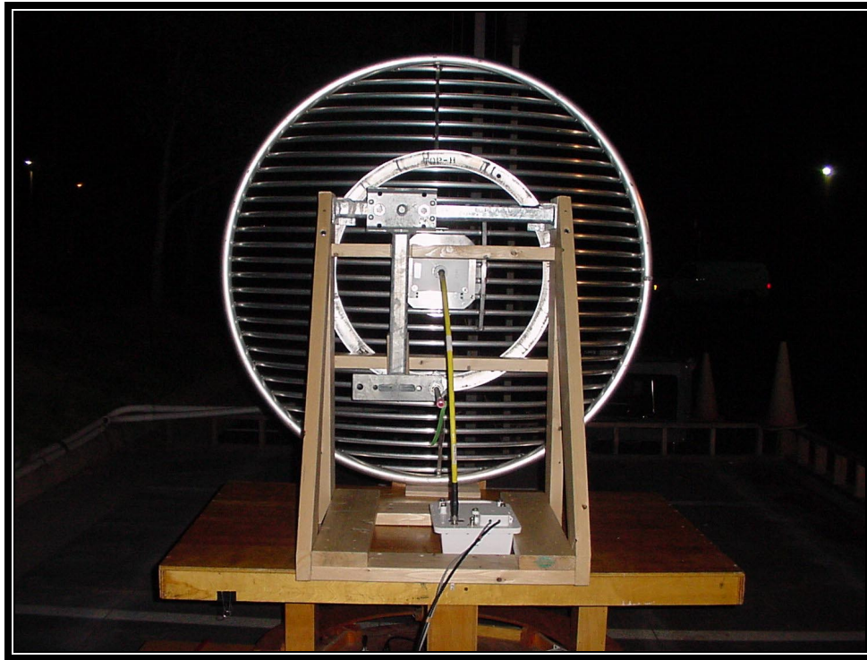
PHOTOGRAPH 1: RADIATED BACK VIEW
