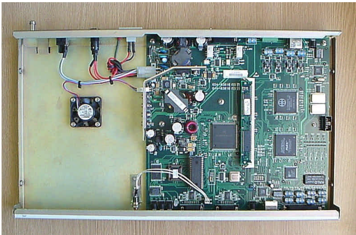
Indoor Unit with Cover Removed
