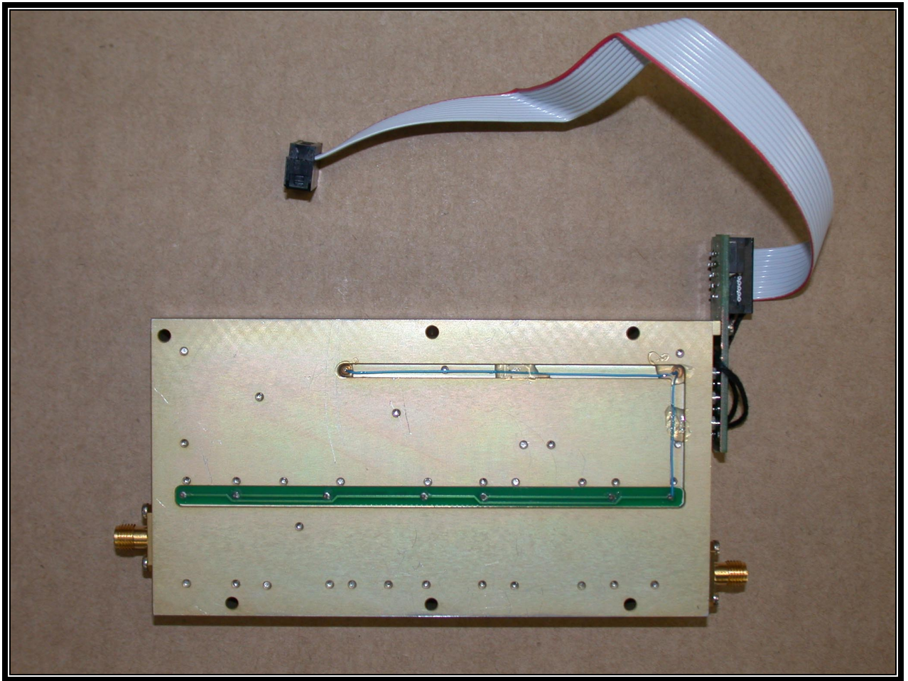
Tx Housing Bottom View
