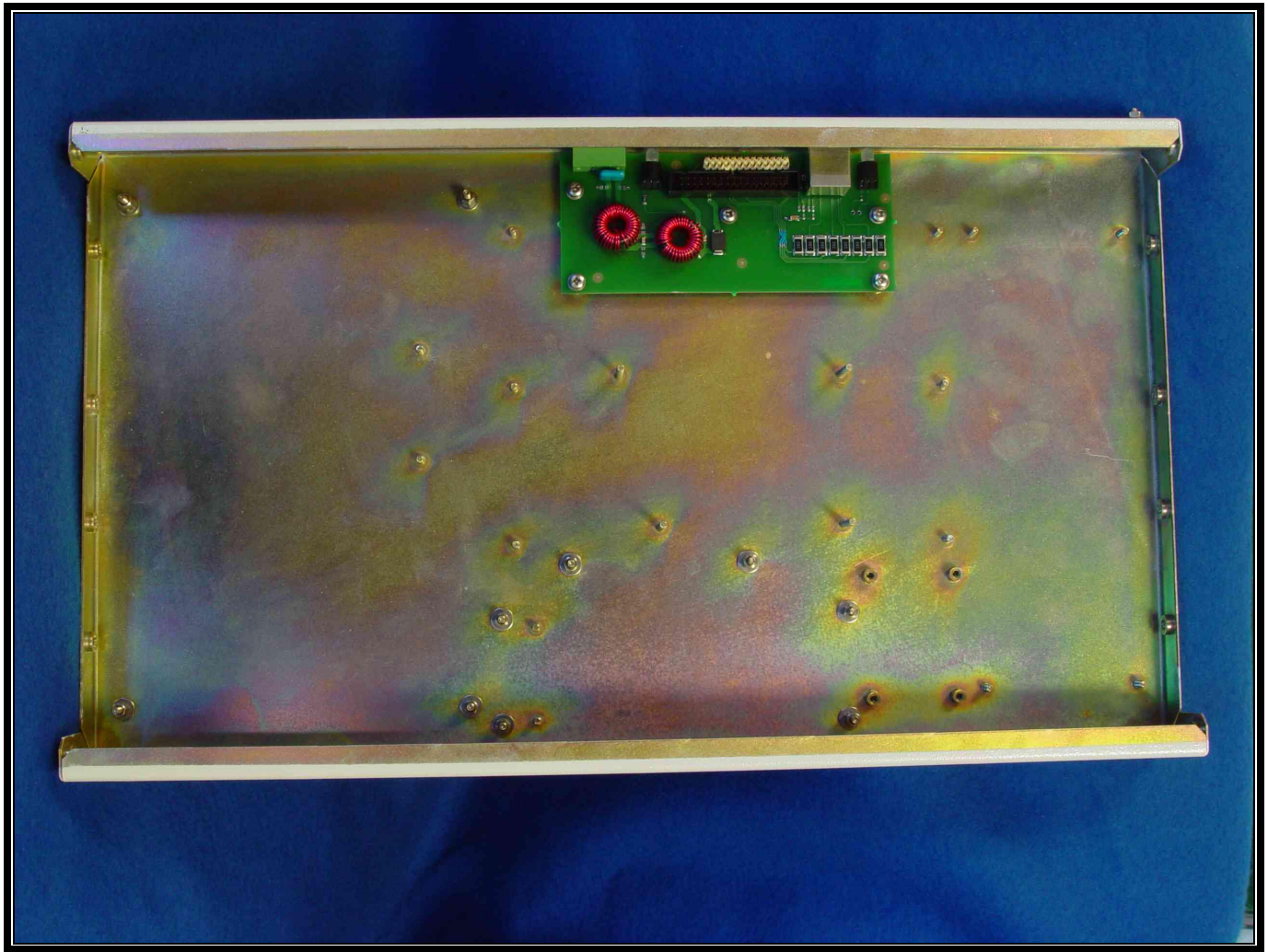
Metal Box with Interface Board Fitted
