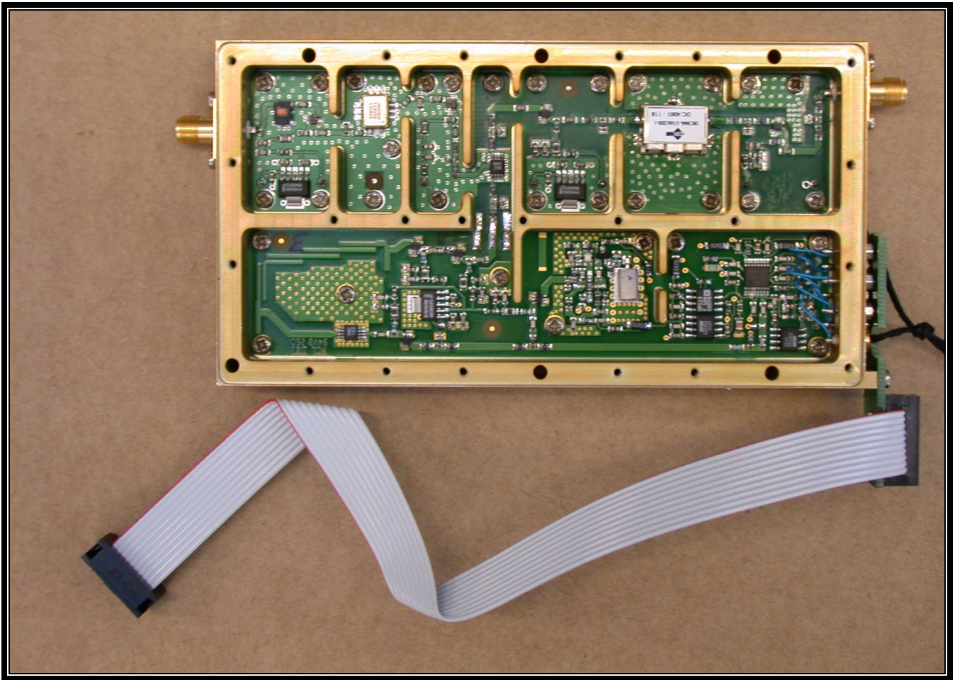
Tx Housing with Lid Removed
