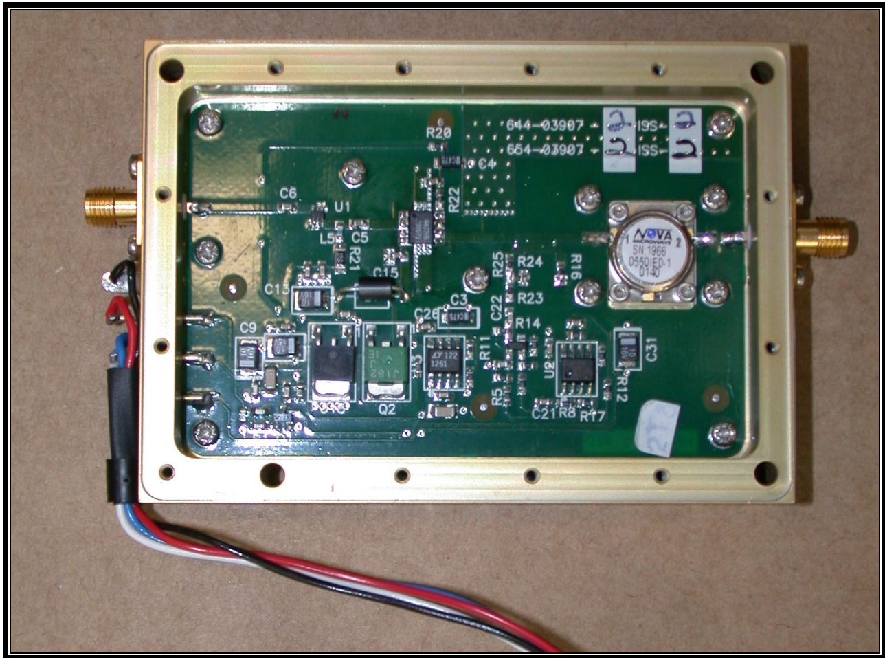
Power Amplifier with Lid Removed
