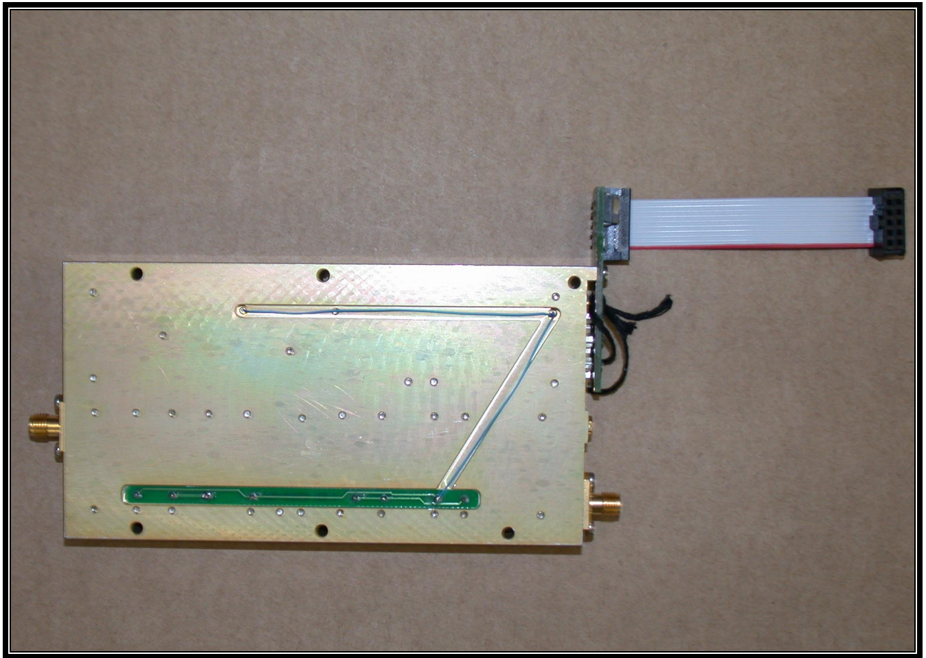
Rx Housing Bottom View
