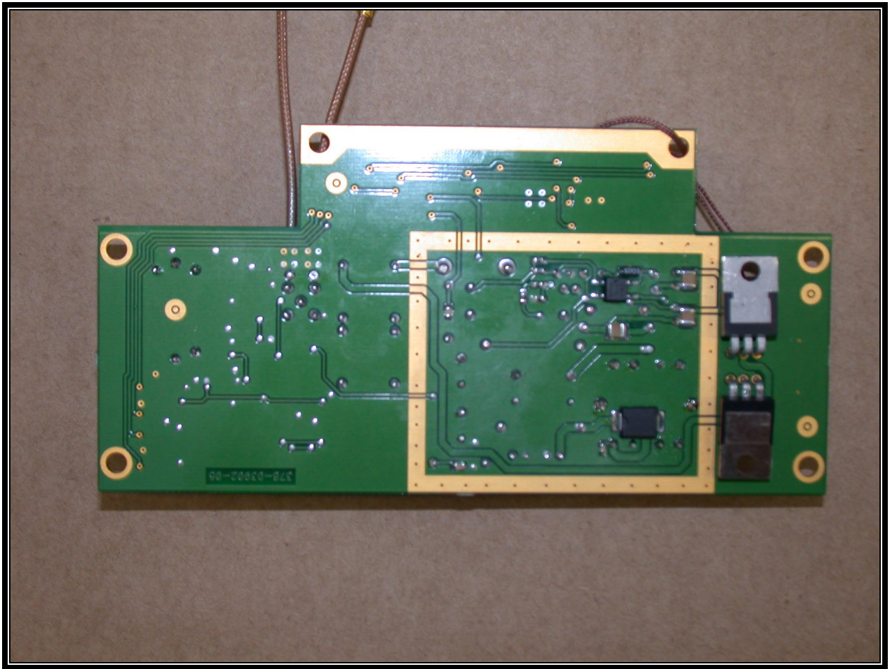
PSU/TCXO Bottom Assembly without Screening Can
