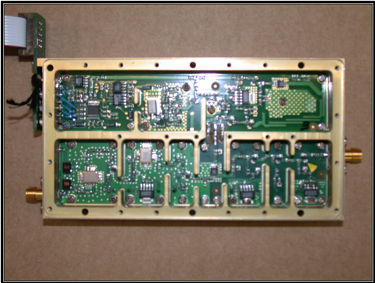
Rx Housing with Lid Removed
