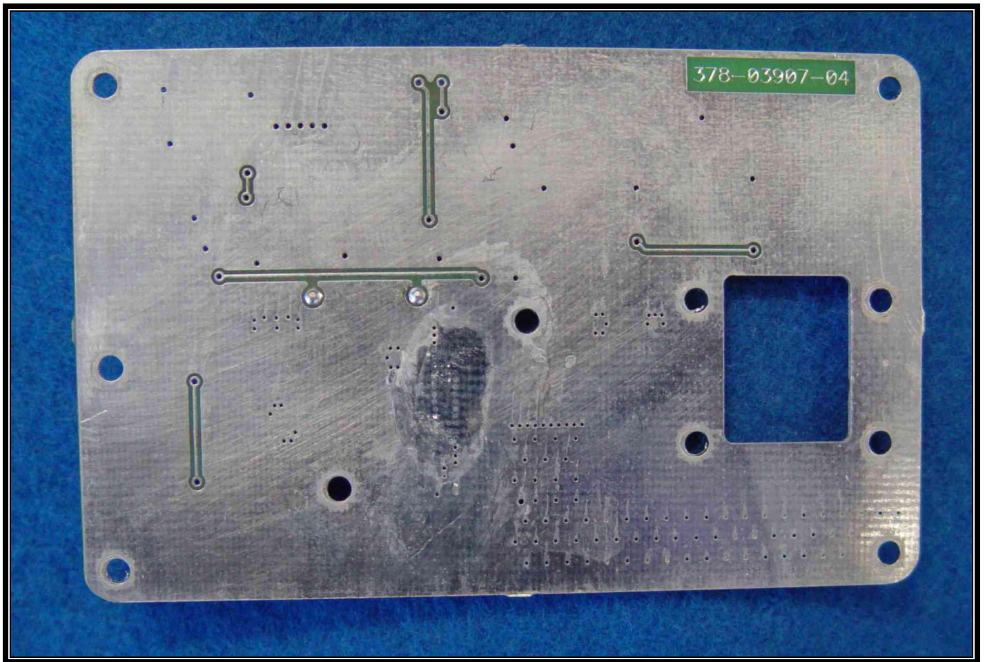
Power Amplifier Board Bottom
