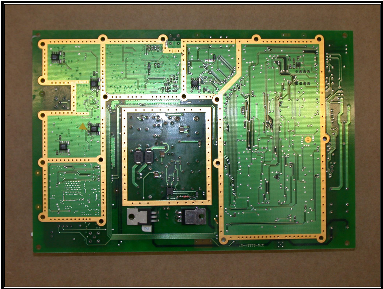
Baseband Processor PCB Bottom without Screening Can
