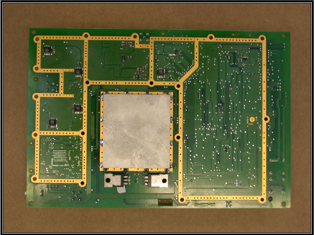
Baseband Processor PCB Bottom with Screening Can
