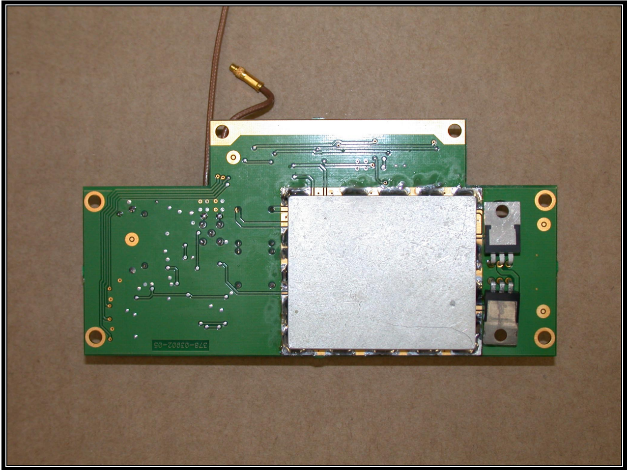
PSU/TCXO Bottom Assembly with Screening Can
