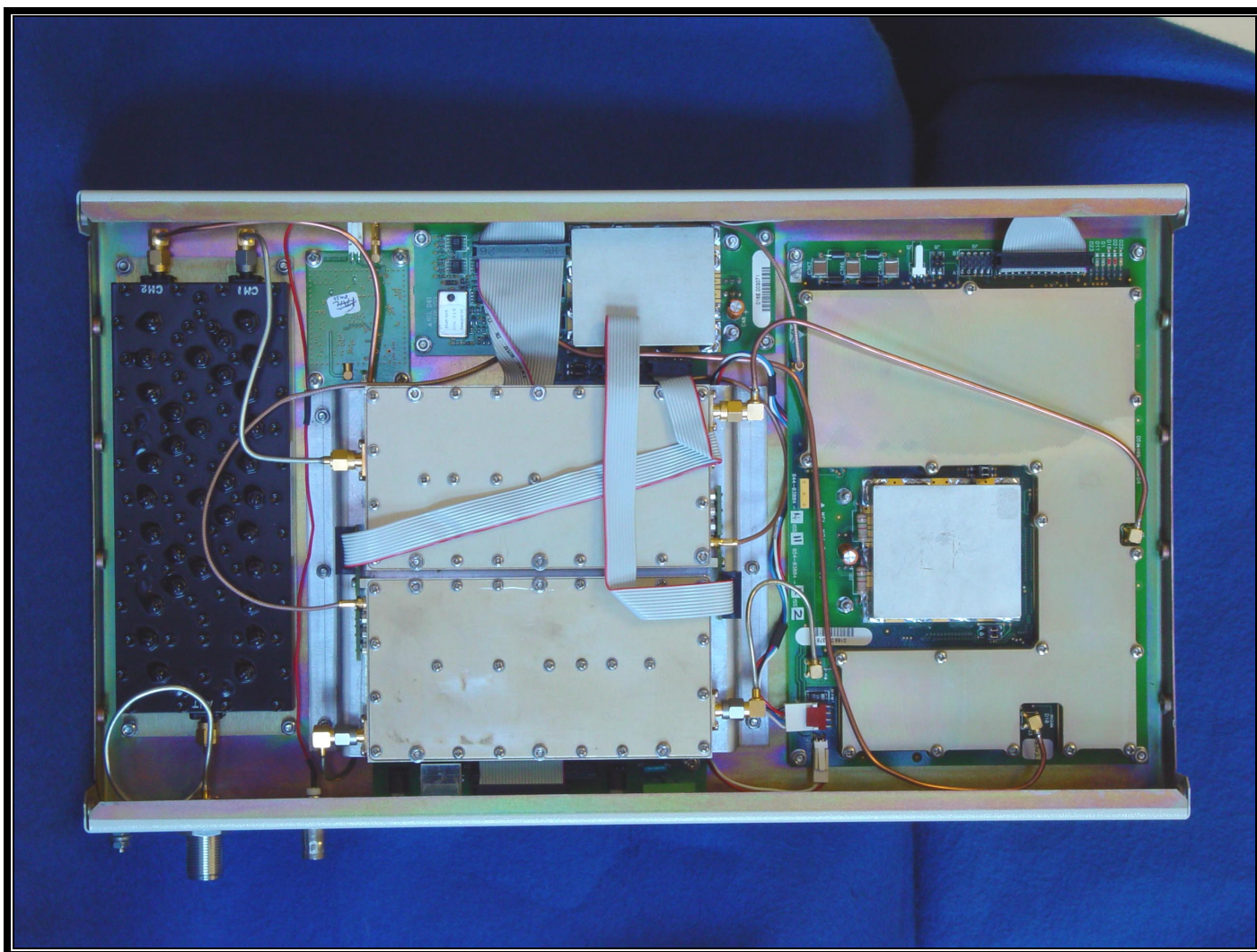
Indoor RF Unit without Top Cover
