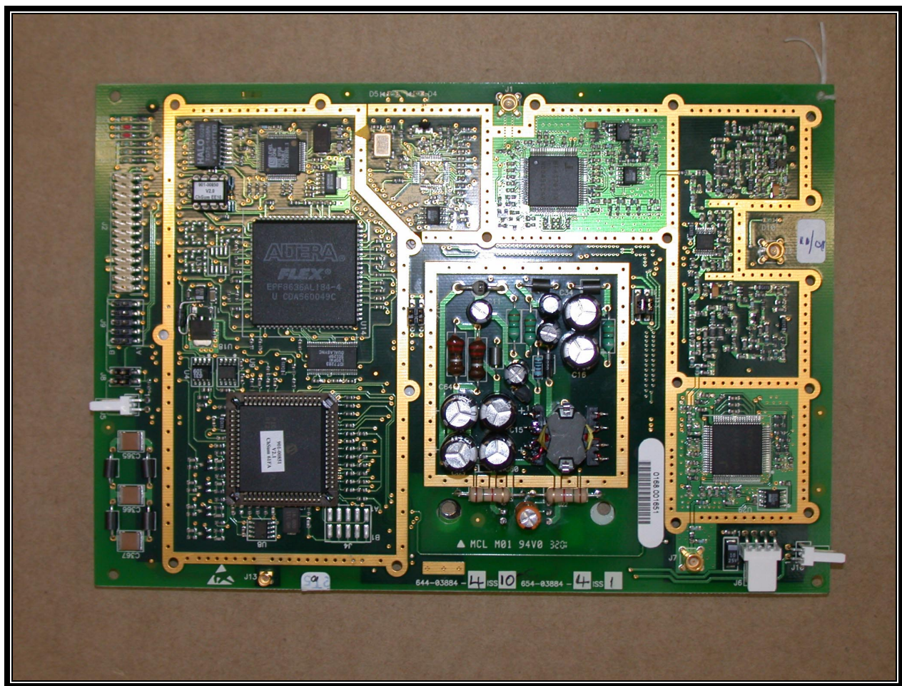
Baseband Processor PCB Top without Screening Can
