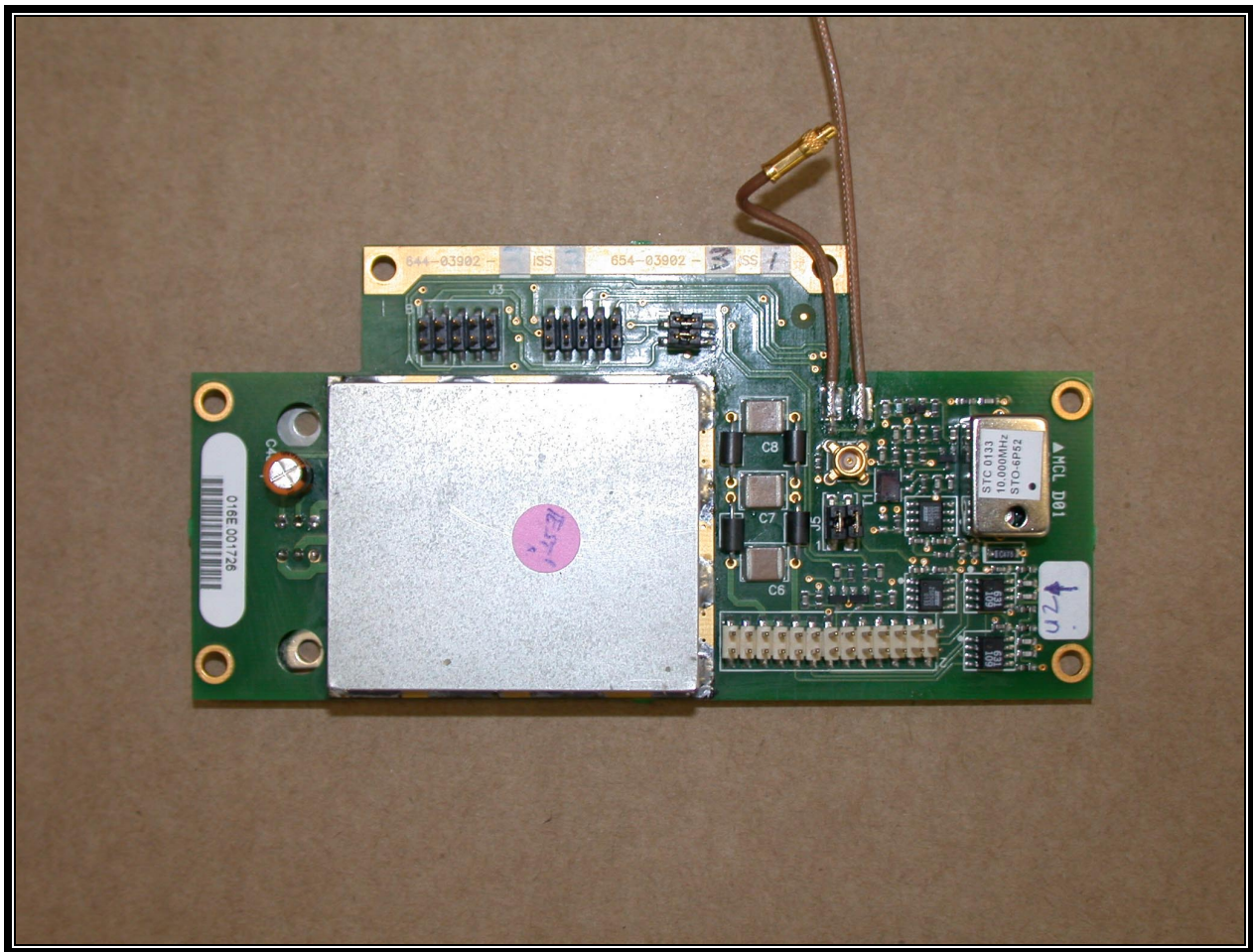
PSU/TCXO Top Assembly with Screening Can
