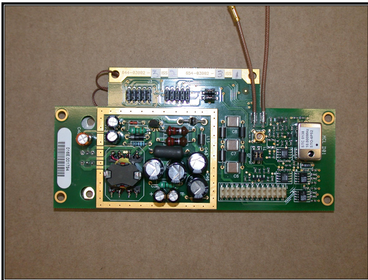
PSU/TCXO Top Assembly without Screening Can
