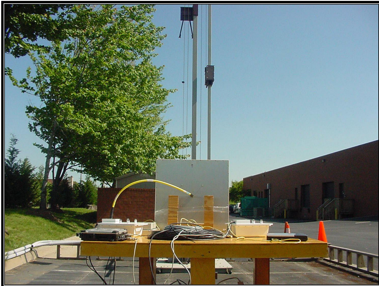
PHOTOGRAPH 4: RADIATED EMISSIONS REAR VIEW – FLAT PANEL ANTENNA
