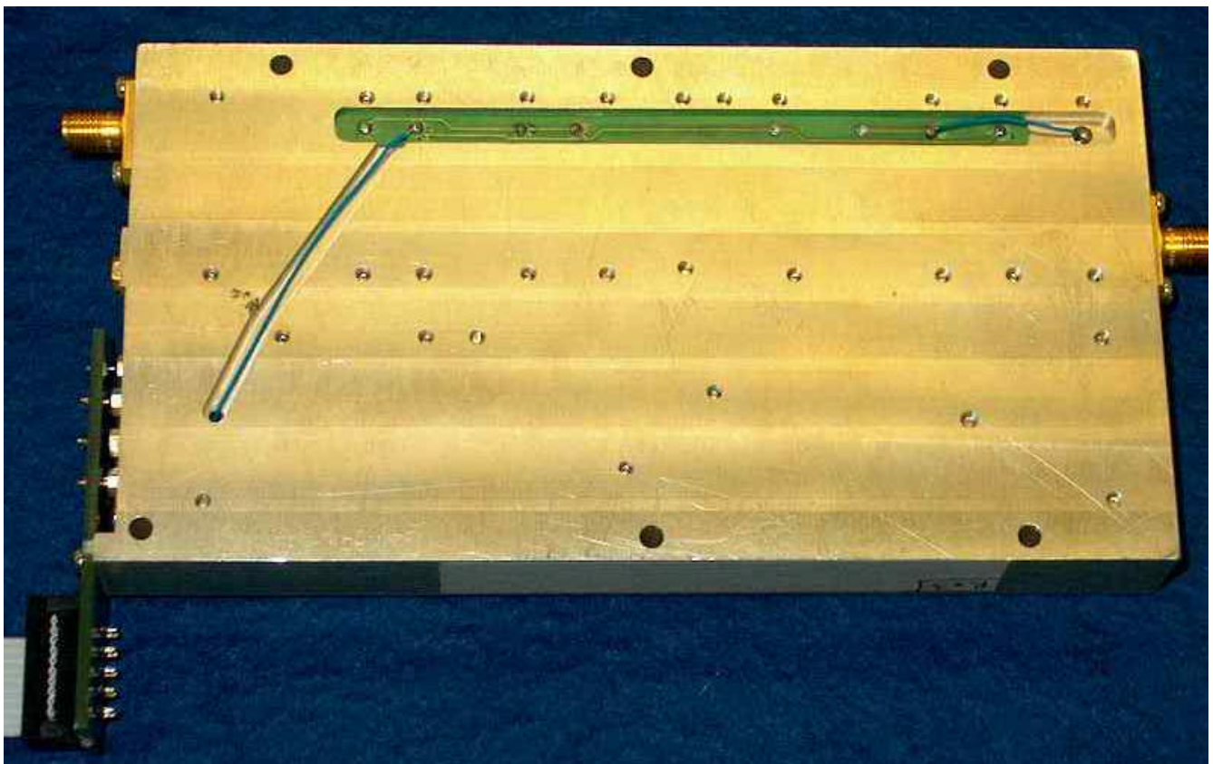
Rx Housing Bottom View
