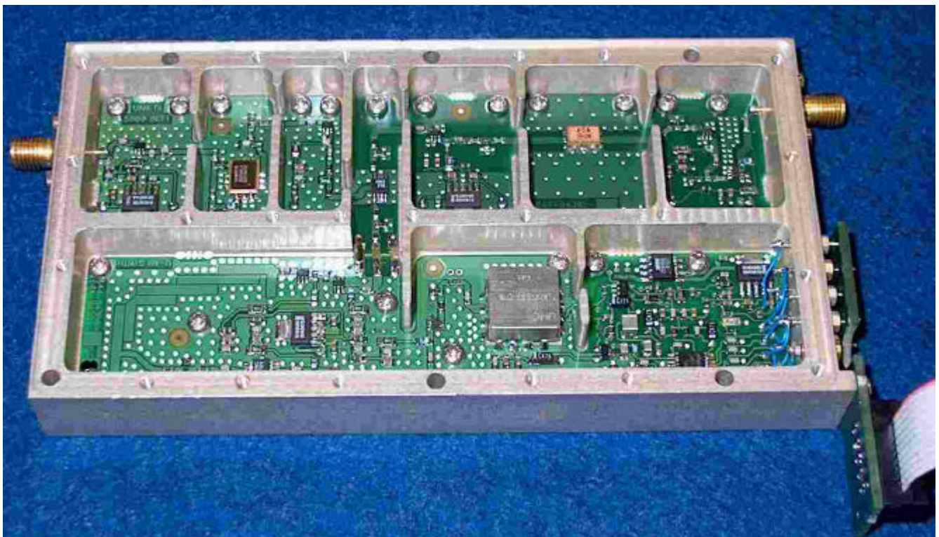
Tx, Synth & Housing
