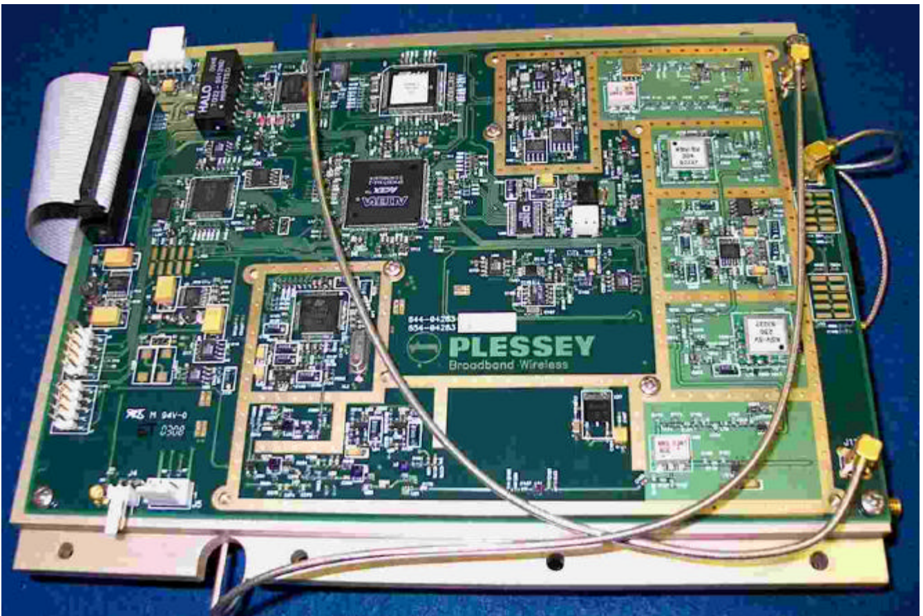
Baseband Processor Top Assembly
