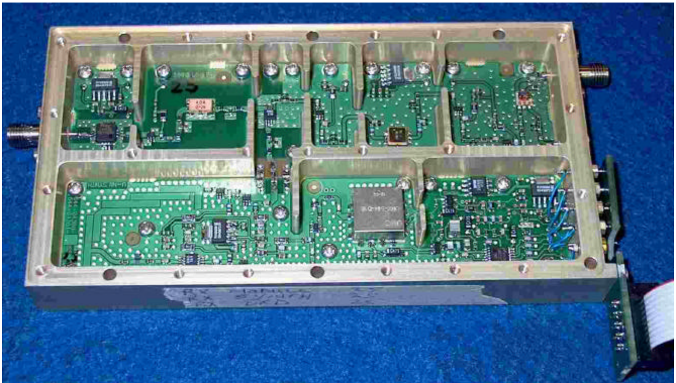
Rx, Synth & Housing
