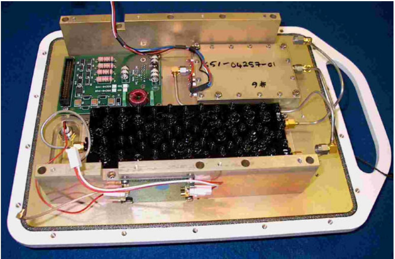
Outdoor Unit with no Baseband Processor Assembly
