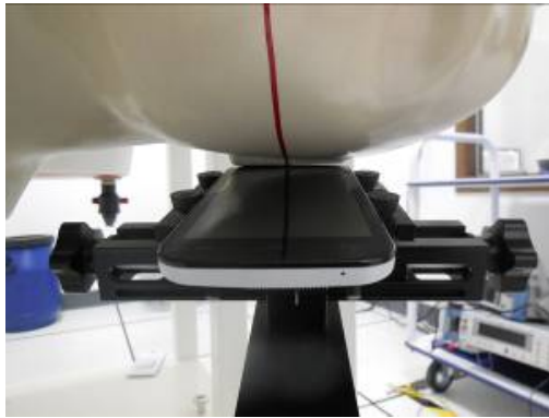
Band850, Band1900, WCDMA Band II/V, WIFI Test Setup Head Touch-Left
