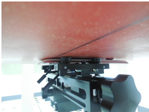
Band850, Band1900, WCDMA Band II/V Test Setup Body Back with gap 0mm
