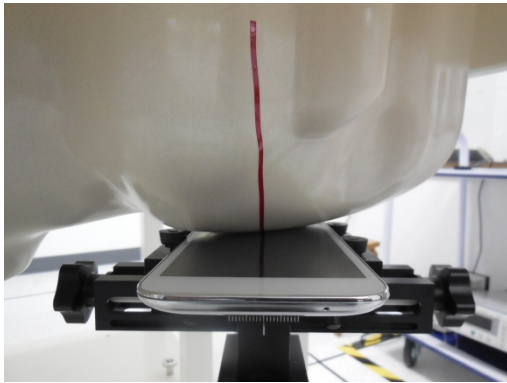
Band850, Band1900, WCDMA Band II/V, WIFI Test Setup Head Touch-Left
