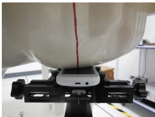
Band850, Band1900, WIFI Test Setup Head Touch-Left
