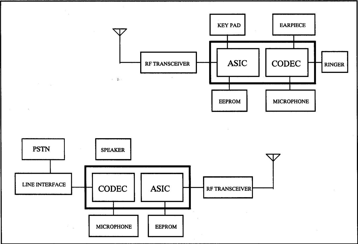
27018GE2-A System Architecture
