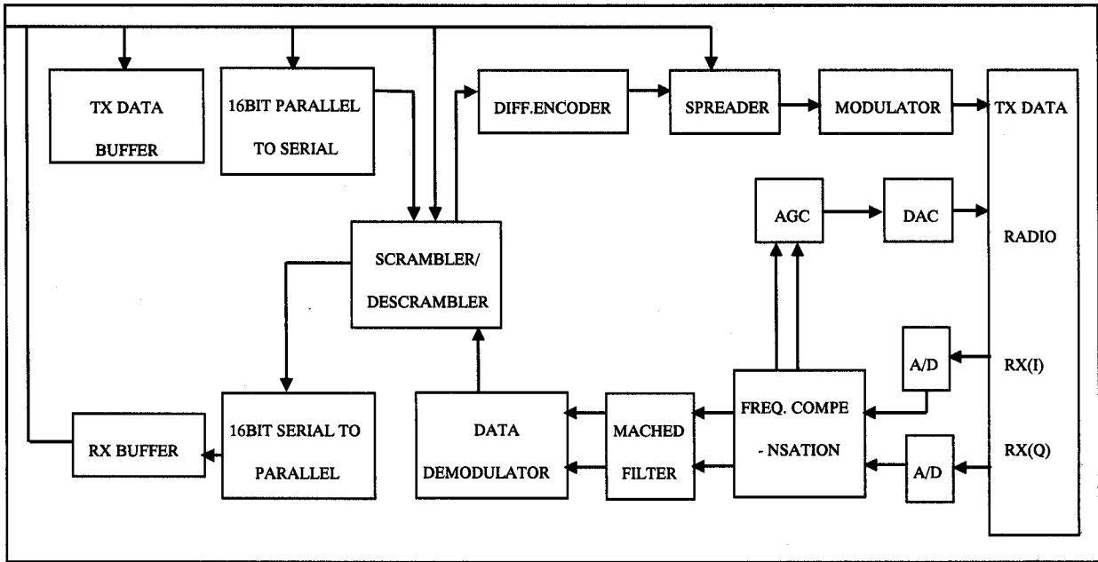
27018GE2-A Spread Spectrum Engine Block
