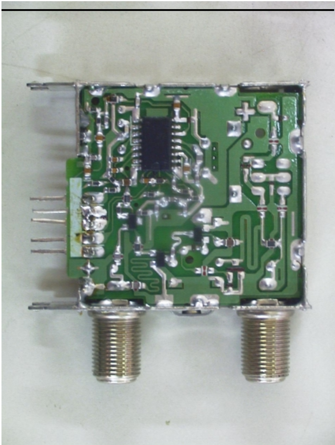
RF Modulator Near
