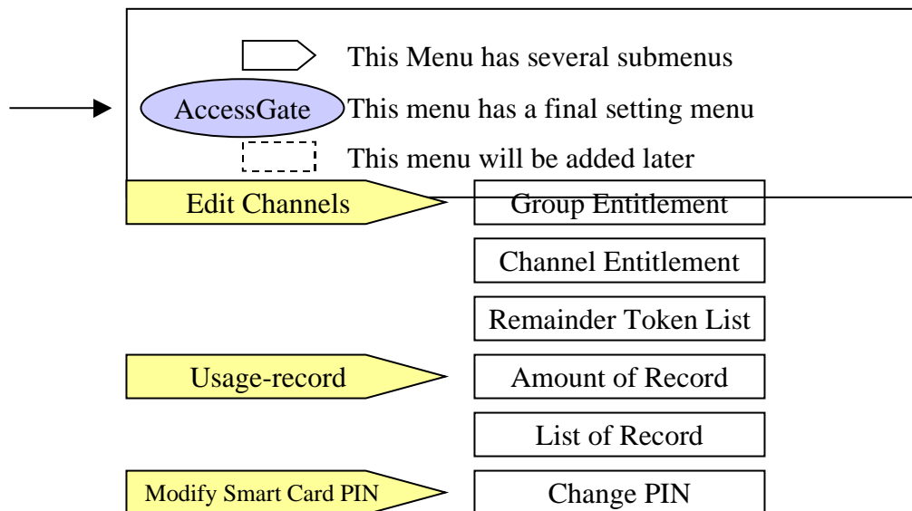
Fig 5. Flow chart of menu system
