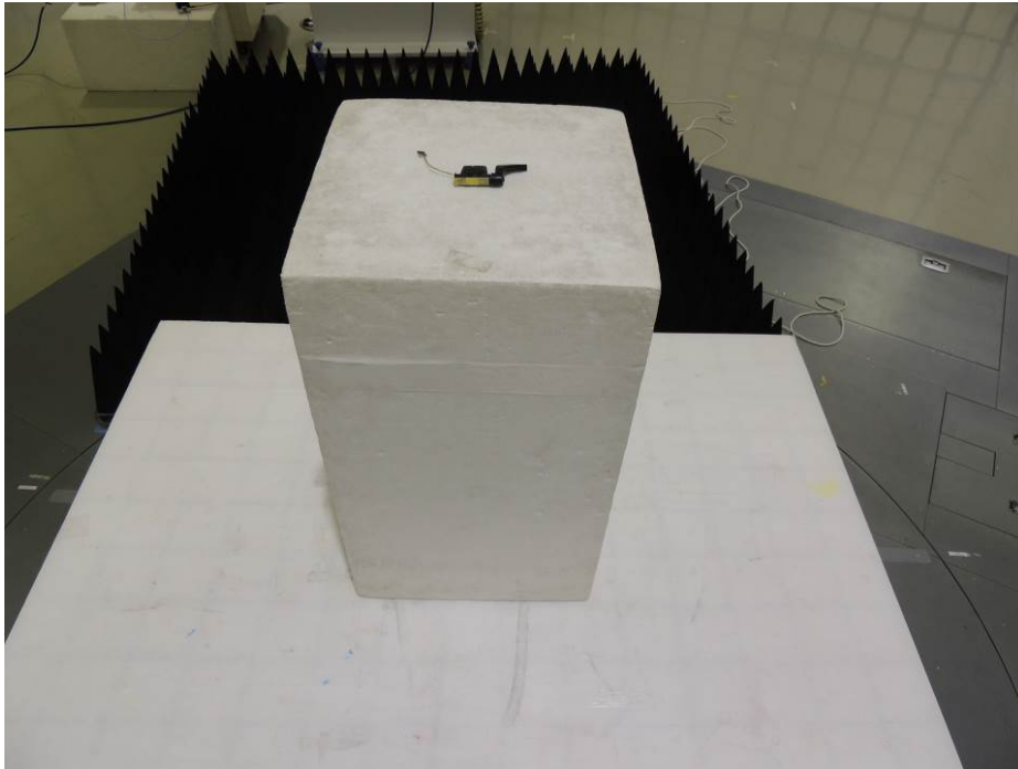
Photograph 3: Set-up for Radiated Emission of Transmitter, GHz Band
