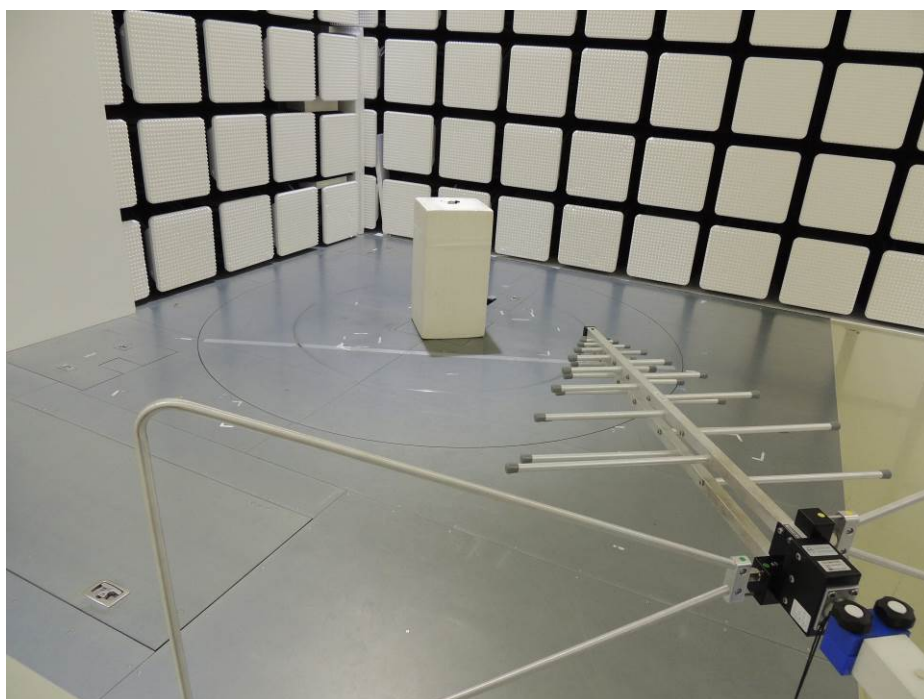
Photograph 2: Set-up for Radiated Emission of Transmitter, MHz Band
