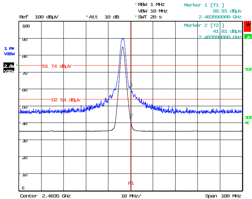
Figure 12: Radiated Emissions at Band Edge, Spectral Diagram, Mode C (2480MHz)
